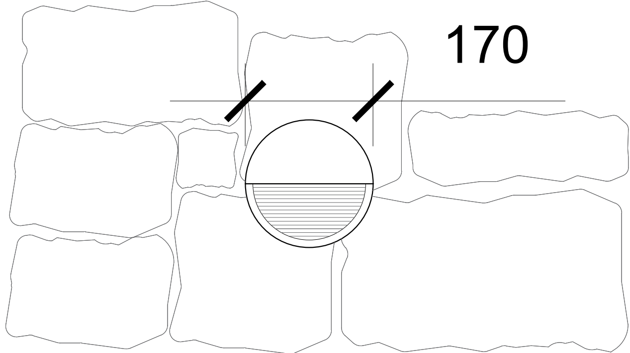
EXTERNAL LIGHTING DETAIL SCALE 1:10
