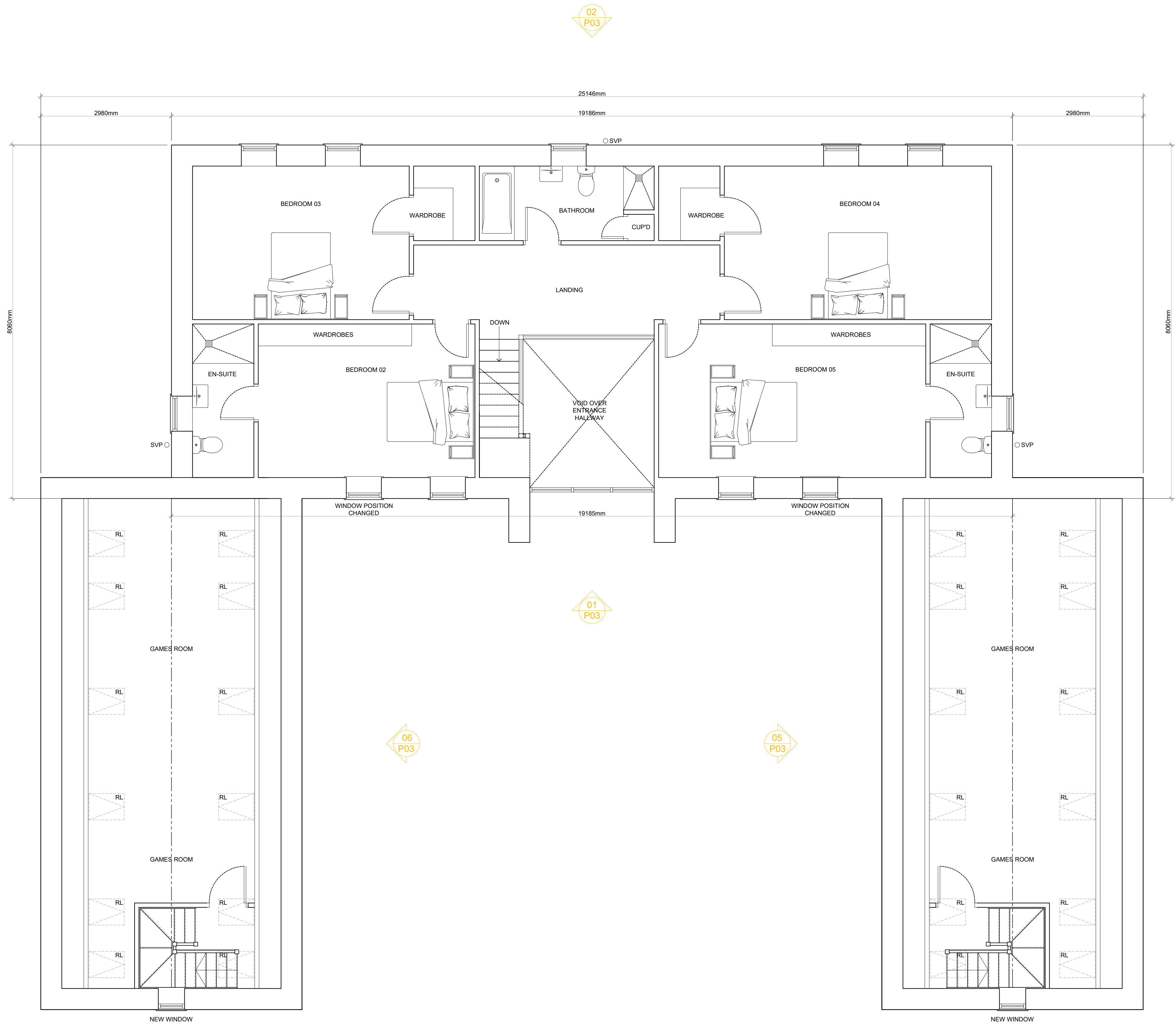
PROPOSED FIRST FLOOR SCALE 1:50
