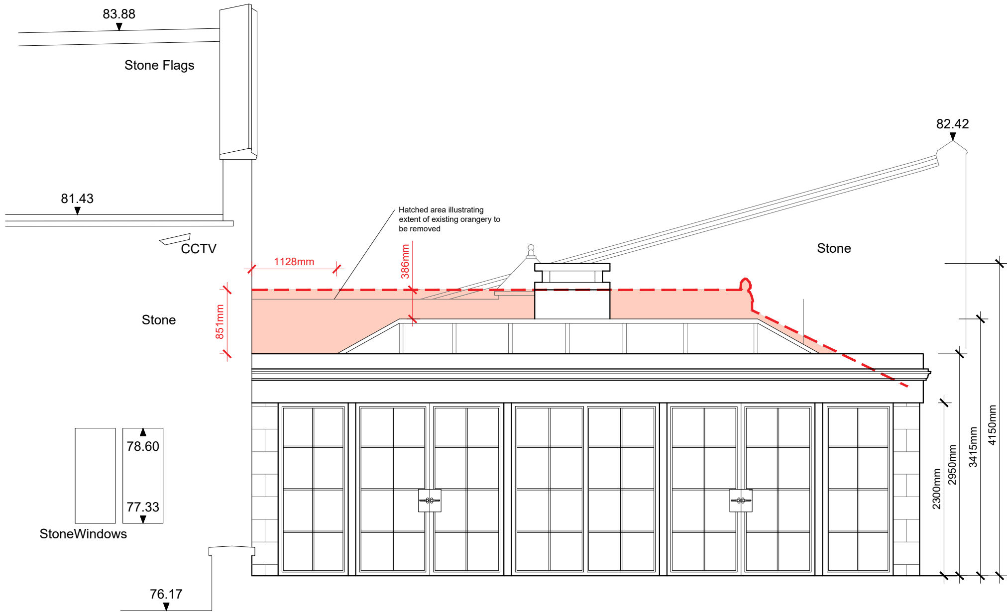
Proposed Extension Elevation Scale 1:50
