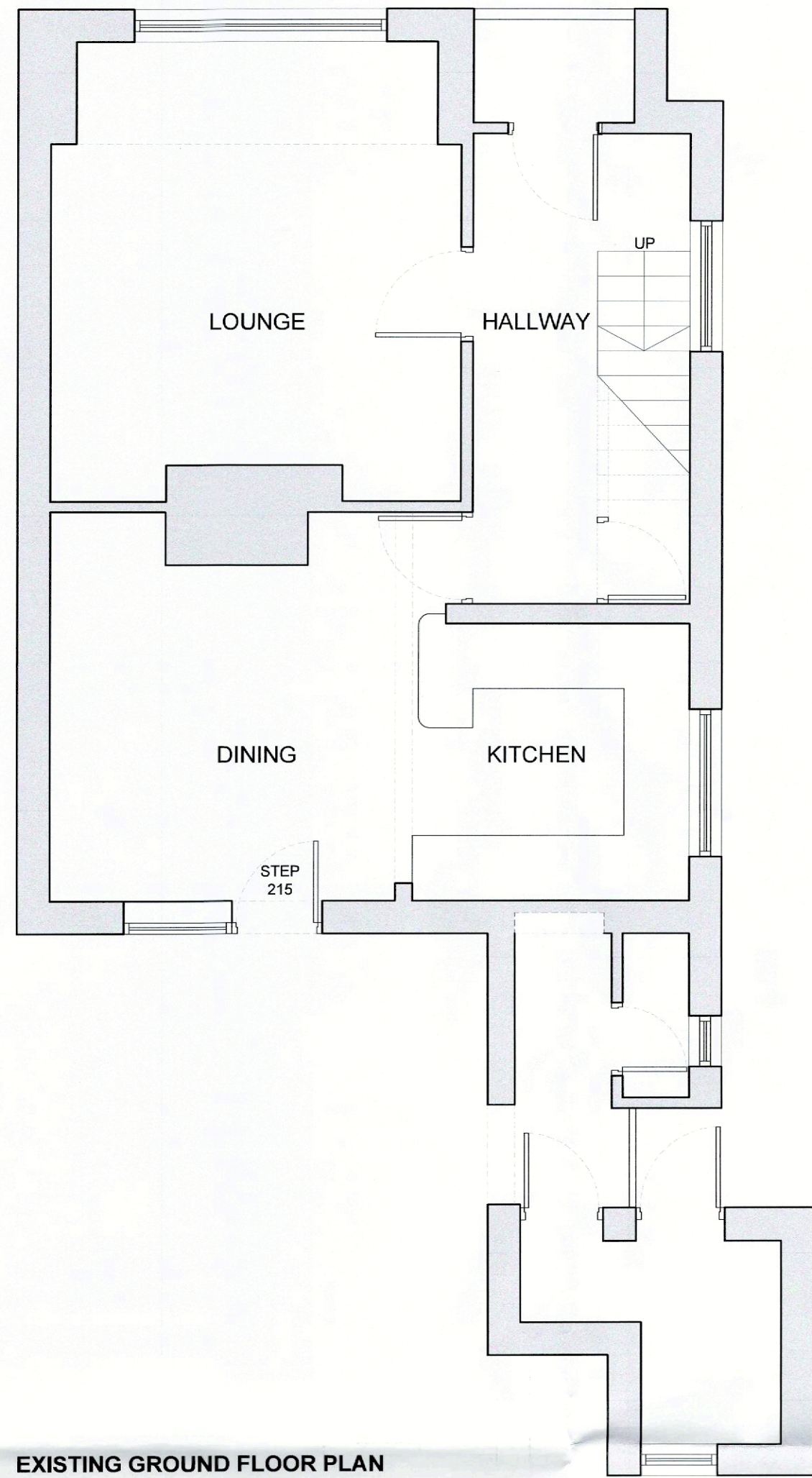
EXISTING GROUND FLOOR PLAN SCALE 1:50 0 1 2 3m
