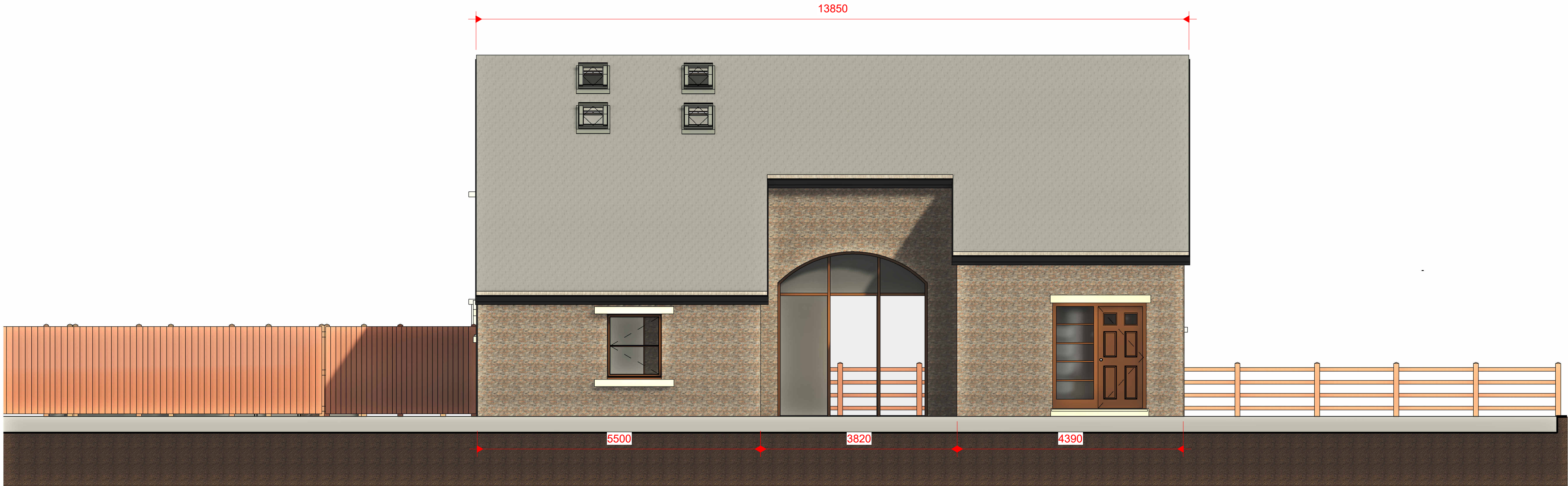
1 PROPOSED SOUTH WEST 1 : 50
