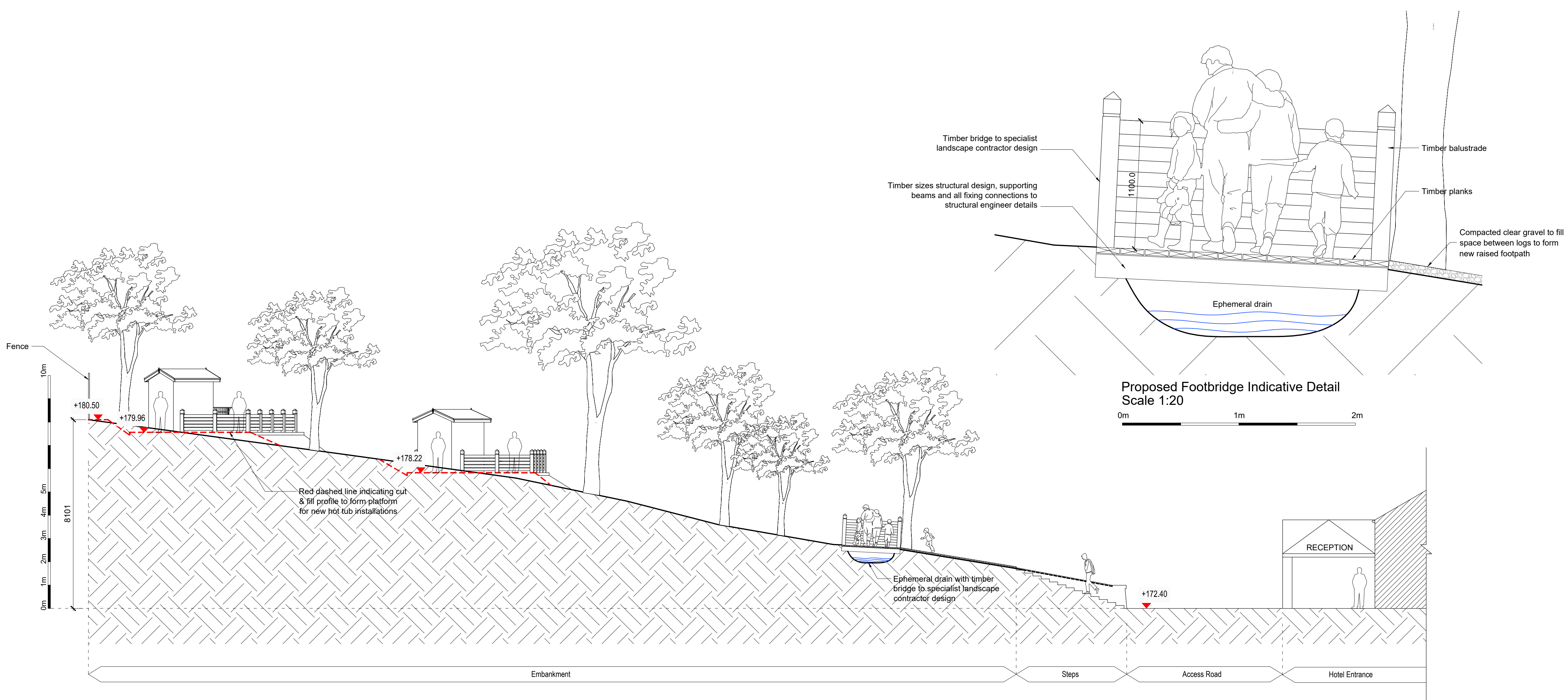
Proposed Site Section S1-S1 Scale 1:100
