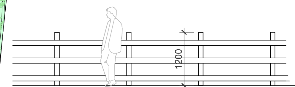
New timber post and rail fence to Southern Boundary 1:50 Scale
