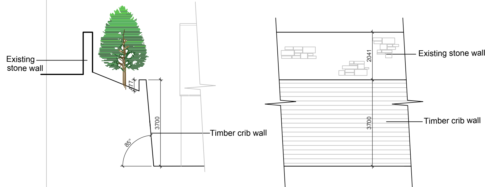
Timber retaining crib wall
