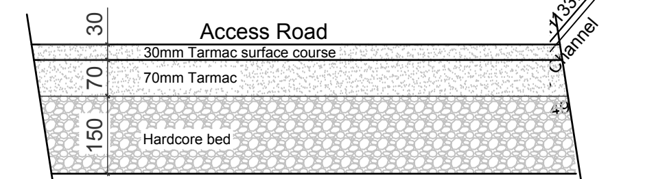
Tarmac Access Road & Parking Area 1:10 Scale
