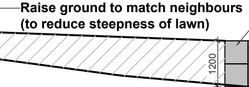
Lego blocks and timber post and rail fence to Southern Boundary Cross Section A, 1:100 Scale
