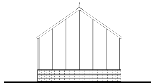
Proposed New Greenhouse North Elevation 1 : 100
