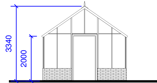
Proposed New Greenhouse South Elevation 1 : 100
