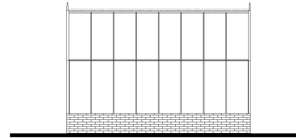
Proposed New Greenhouse East Elevation 1 : 100
