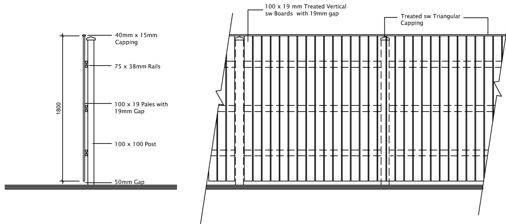
Type A - 1.8m high Close Boarded Timber Fence
