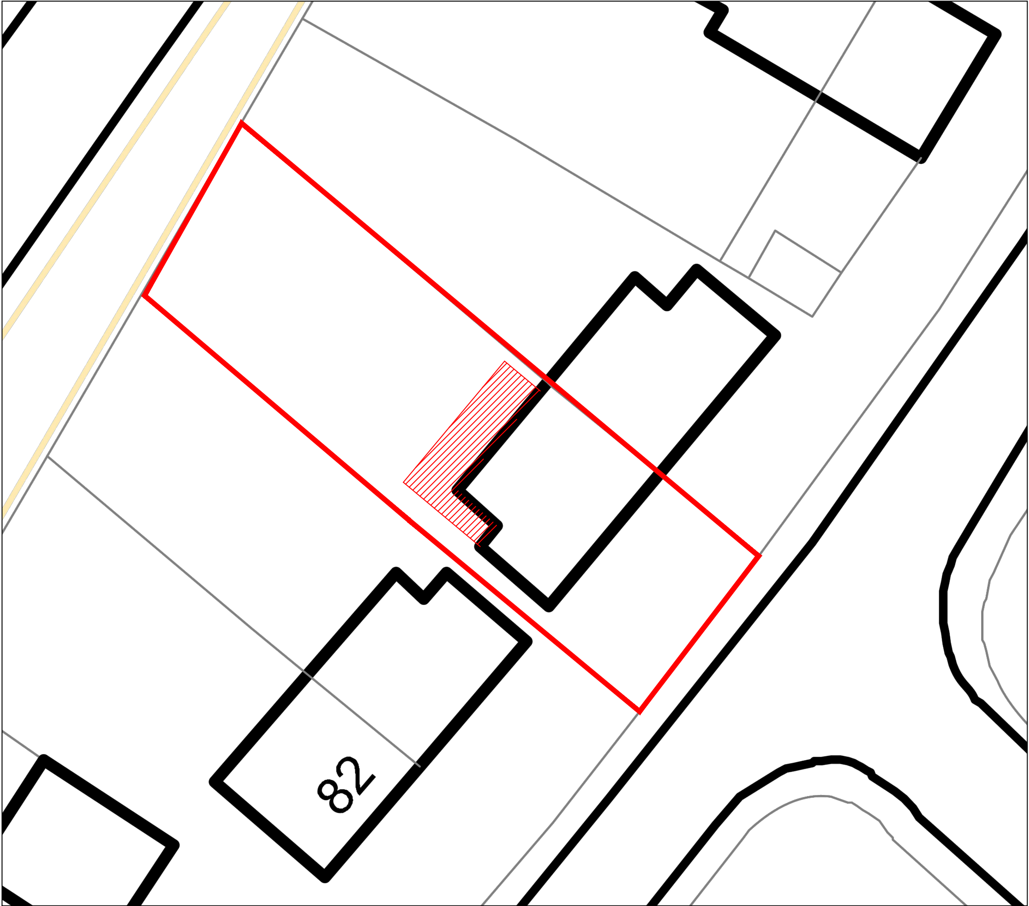
Block Plan (1:200)
