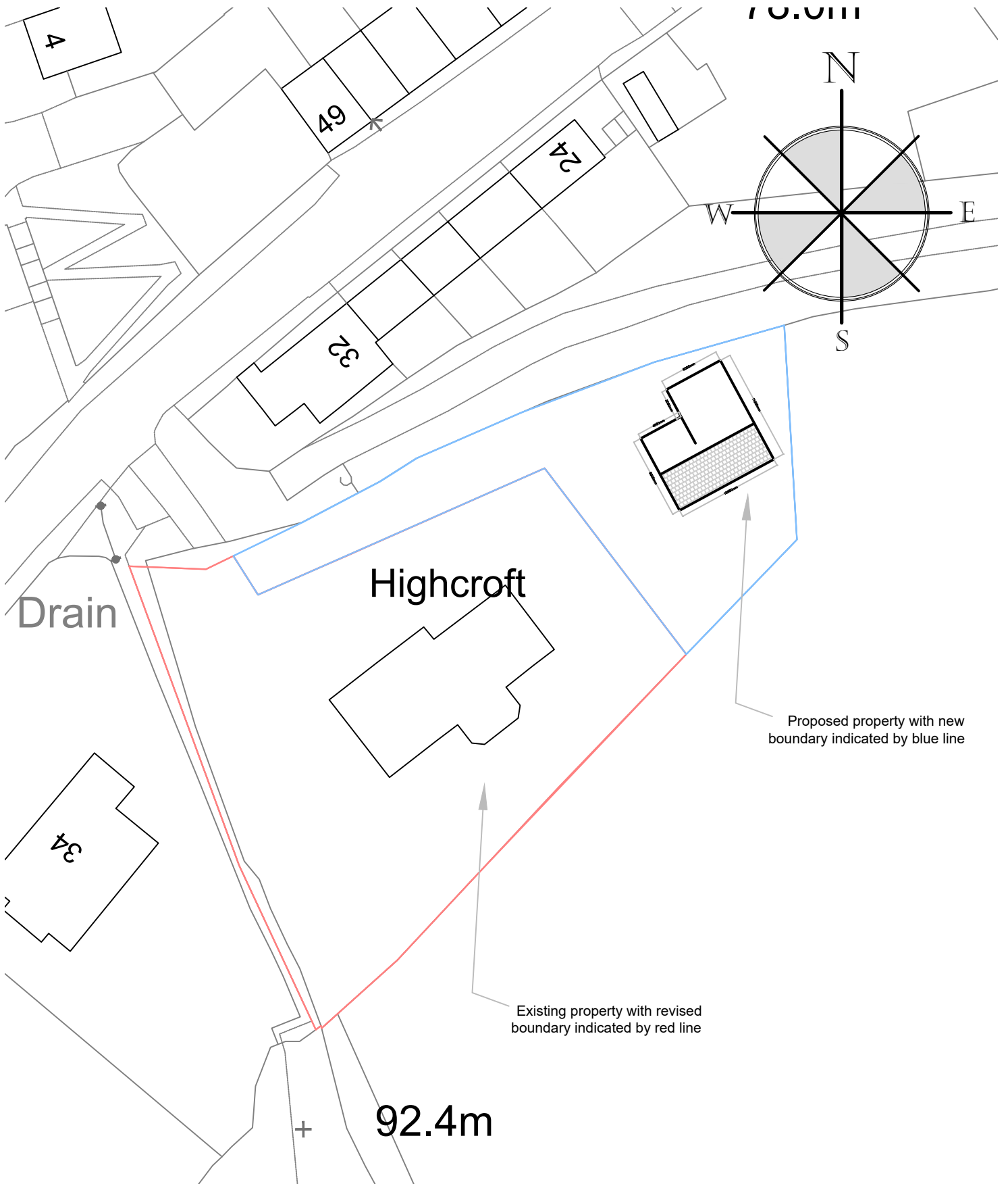
Proposed Site Plan @ 1:500
