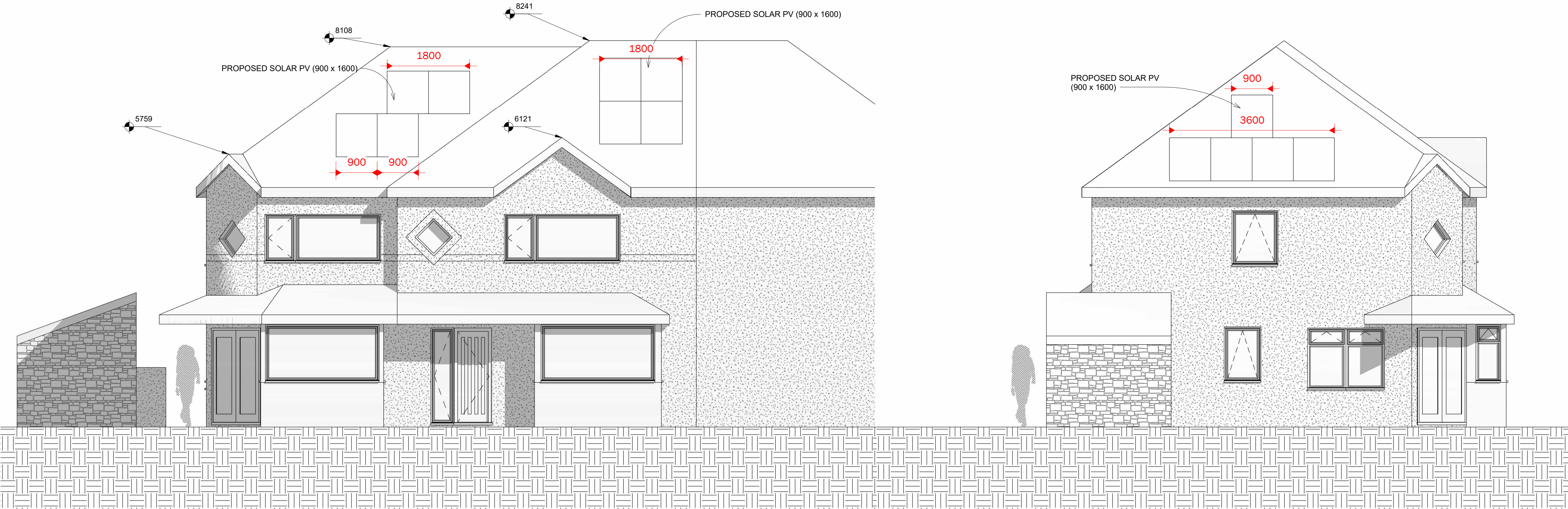
2 PROPOSED SOUTH 1 : 50
