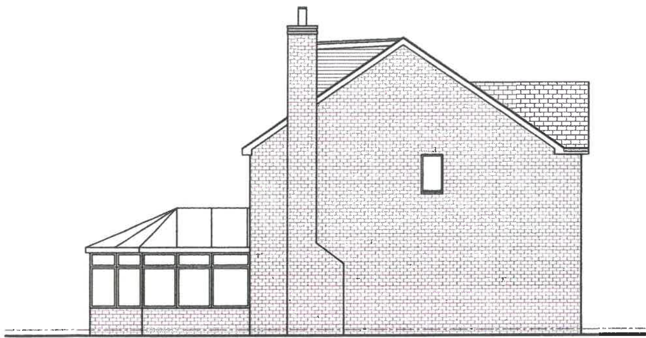
Existing Elevation - Side Scale 1:100
