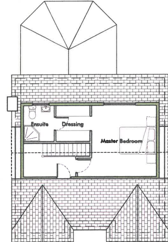
Existing Plan - Second Floor Scale 1:100
