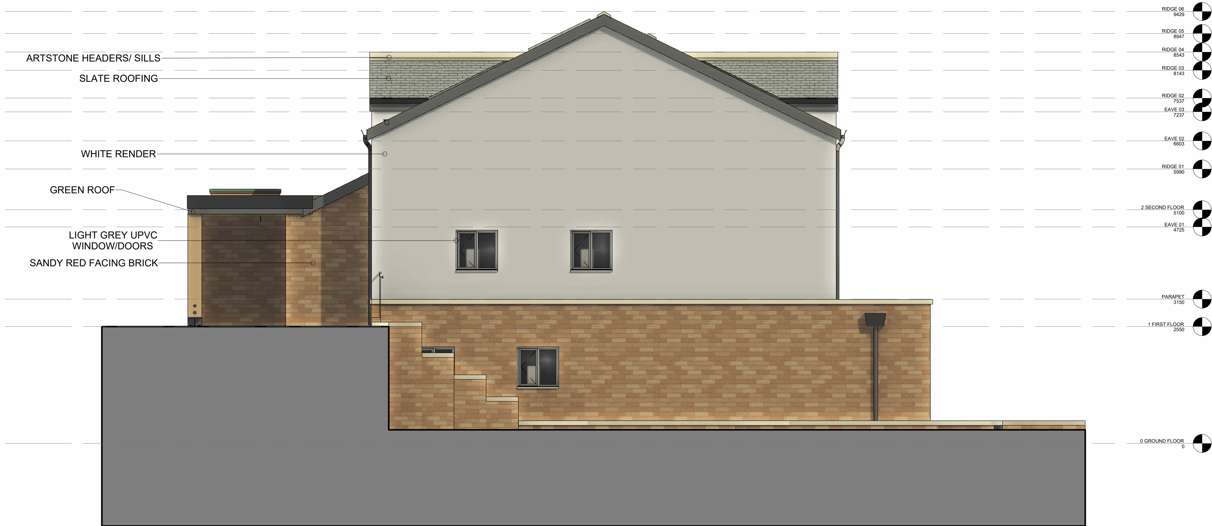
PROPOSED SIDE ELEVATION 2
