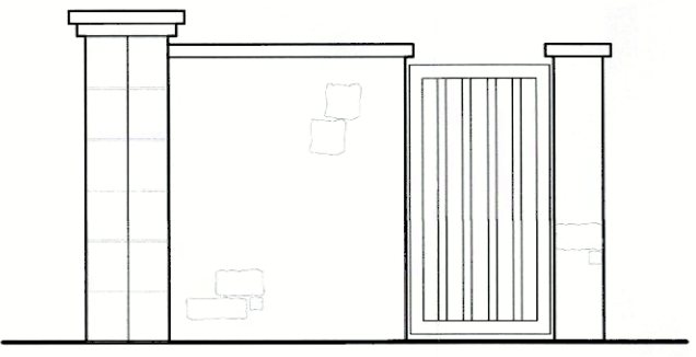
Pedestrian Access Gate Front Elevation (View 01) 1:50 Scale
