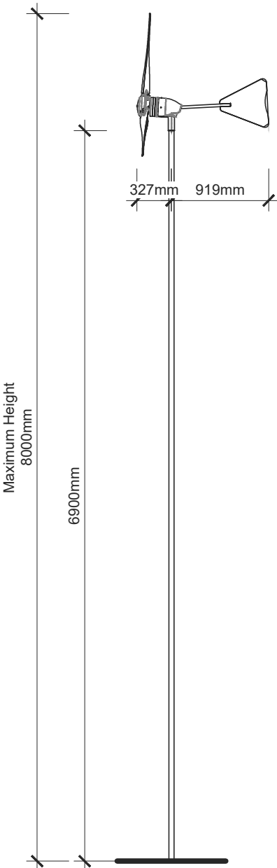
WIND TURBINE AF1 SIDE ELEVATION Scale 1:50
