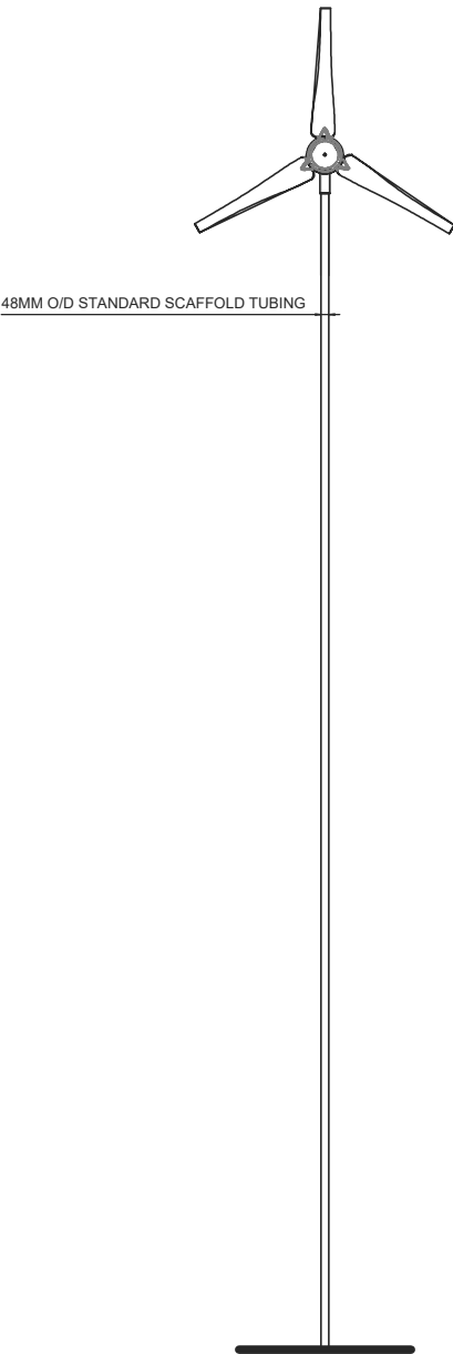
WIND TURBINE AF1 FRONT ELEVATION Scale 1:50
