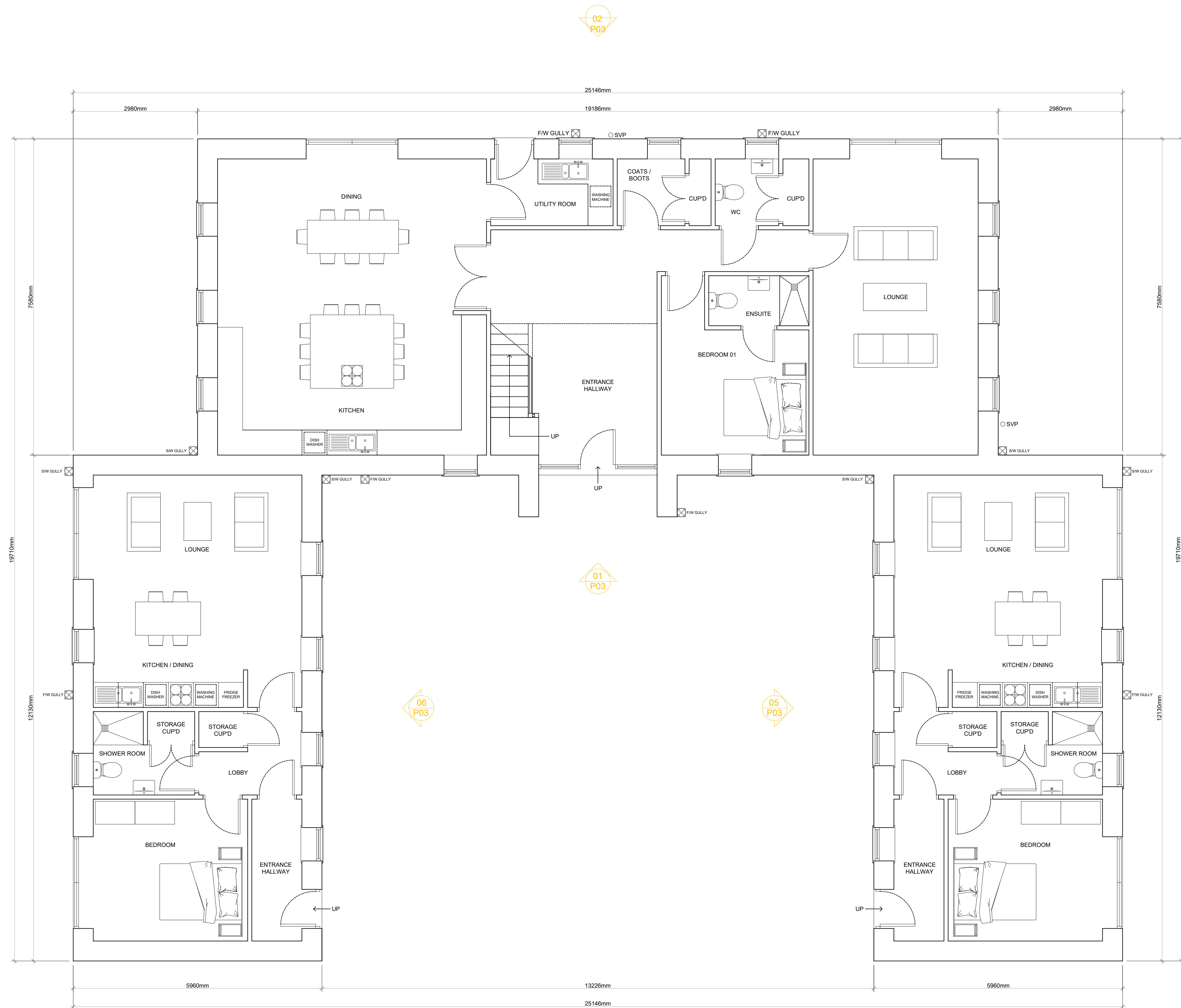
EXISTING GROUND FLOOR
