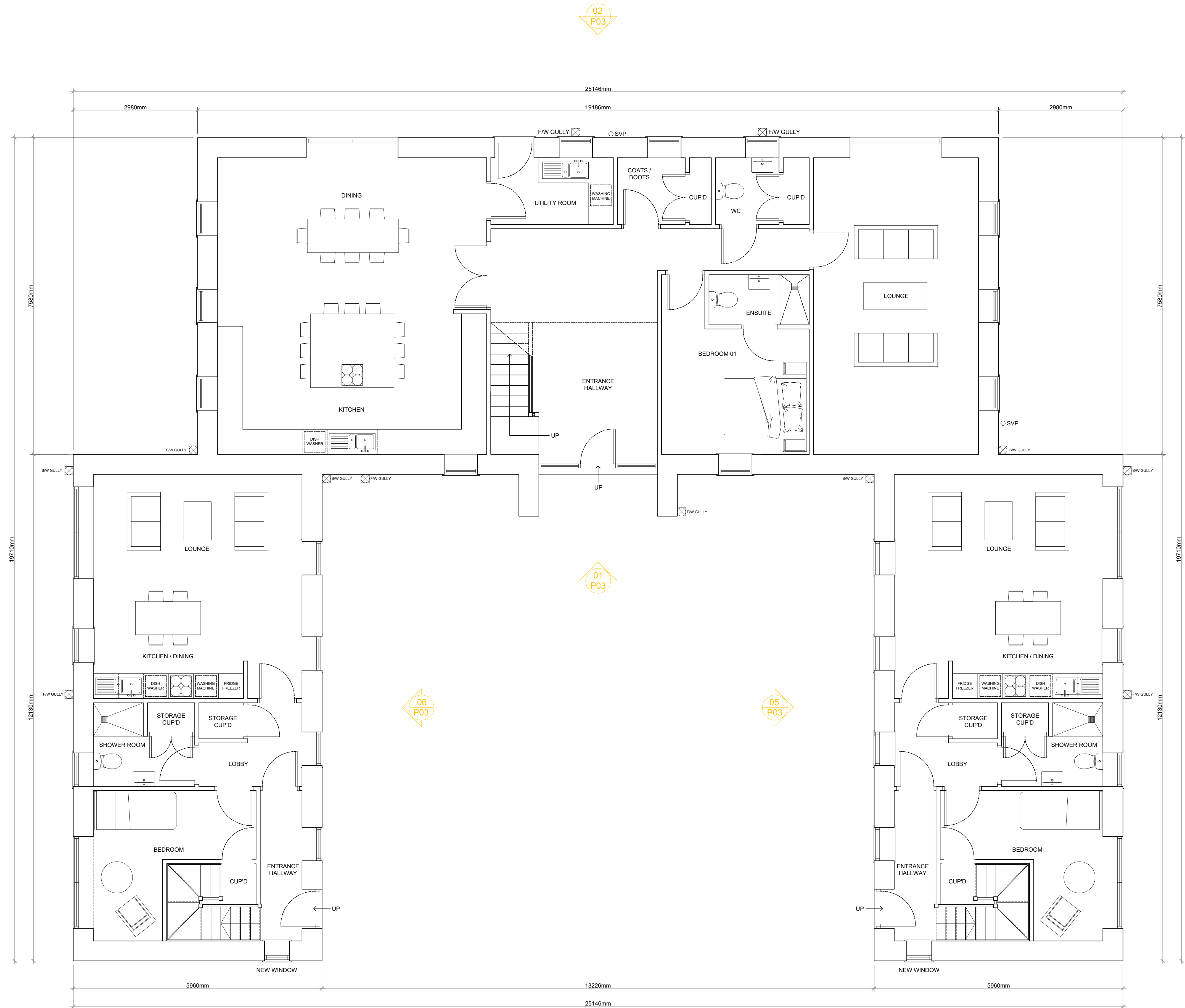
PROPOSED GROUND FLOOR SCALE 1:50 0 1 2 3m
