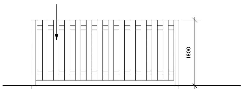
B proposed elevation Scale: 1:50
