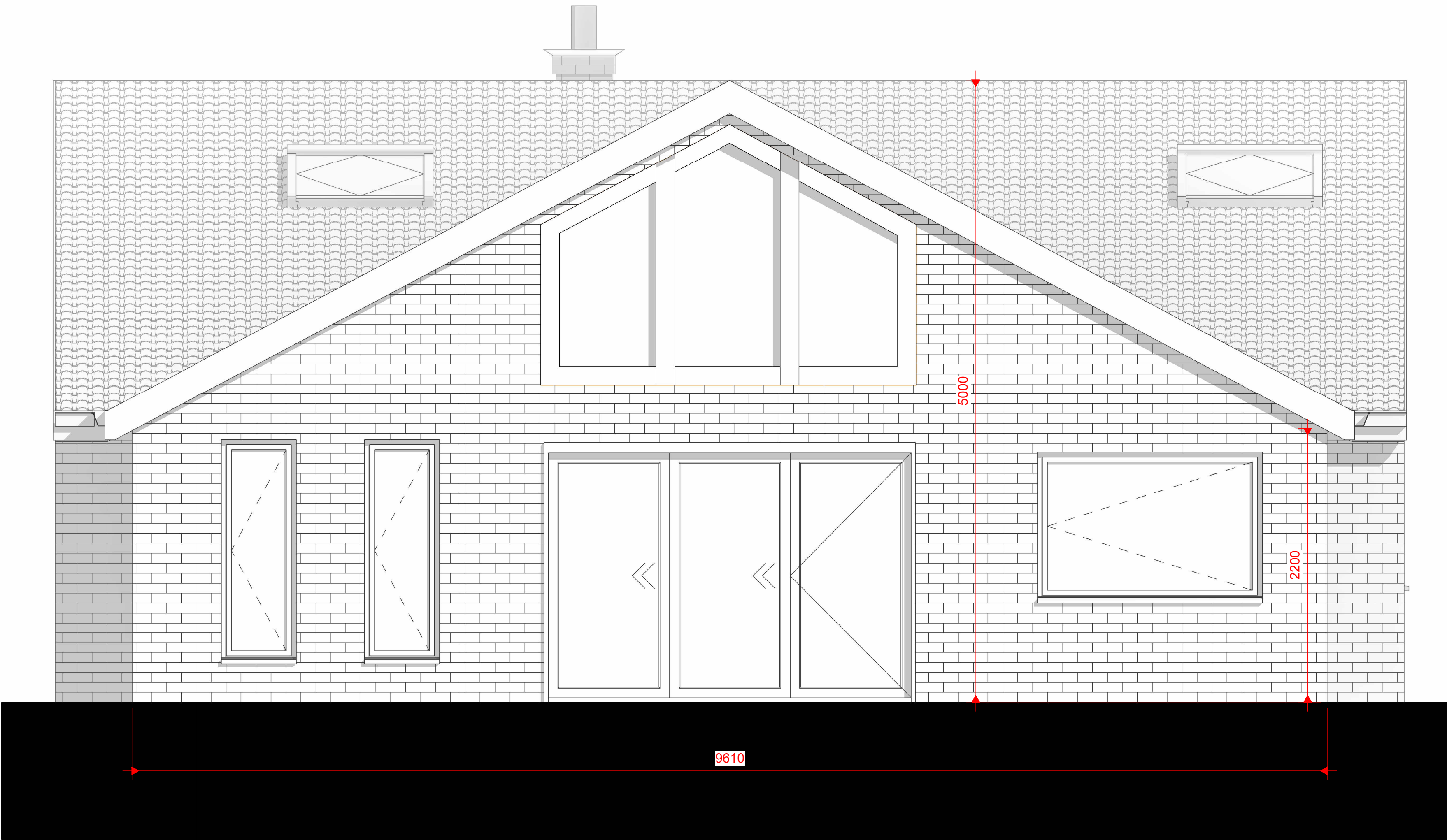
1 PROPOSED NORTH 1 : 25
