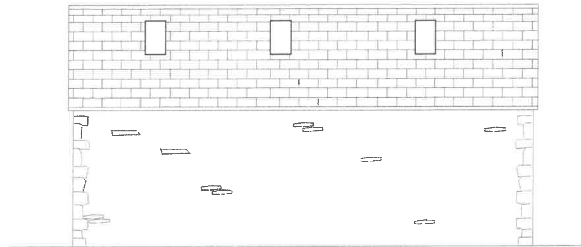
East Elevation
