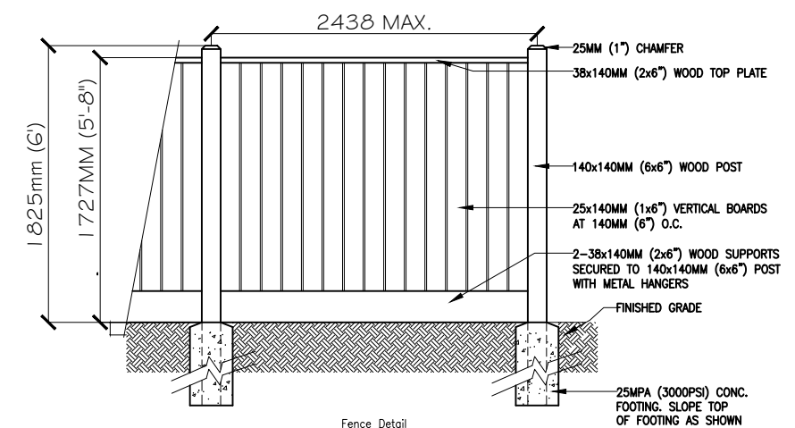
Fence Detail
