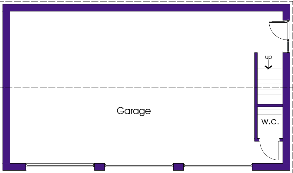
Plan Ground scale 1:100 0 1 2 3 4 5m
