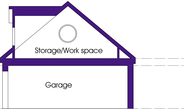
Typical Section scale 1:100
