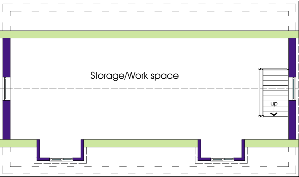
Plan First scale 1:100 0 1 2 3 4 5m
