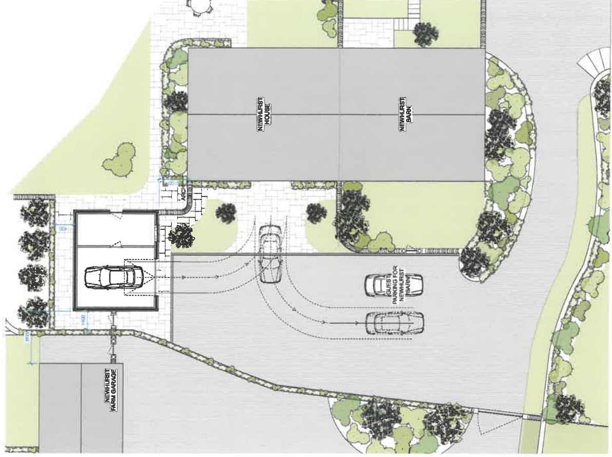
6 Plan - Site Location & Vehicle Movement Scale: 1/8" = 1'-0" @ A1 1/200 @ A3
