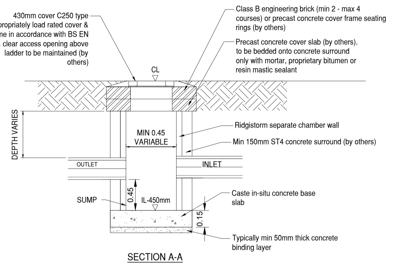
Ridgistorm Separate Catchpit NTS
