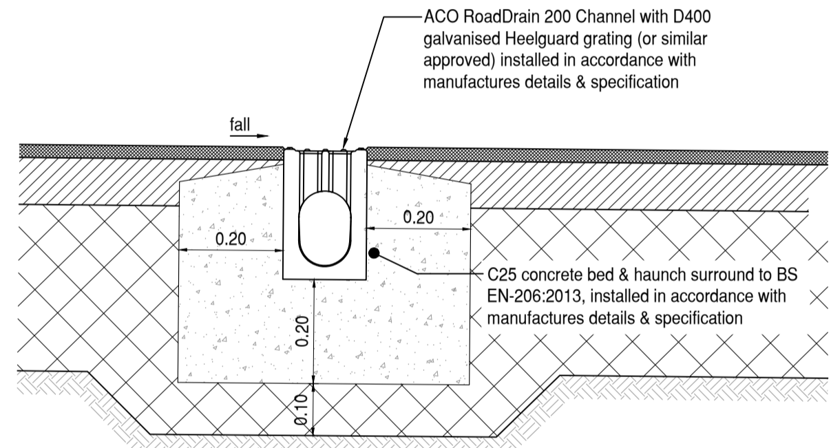
ACO RoadDrain Detail NTS
