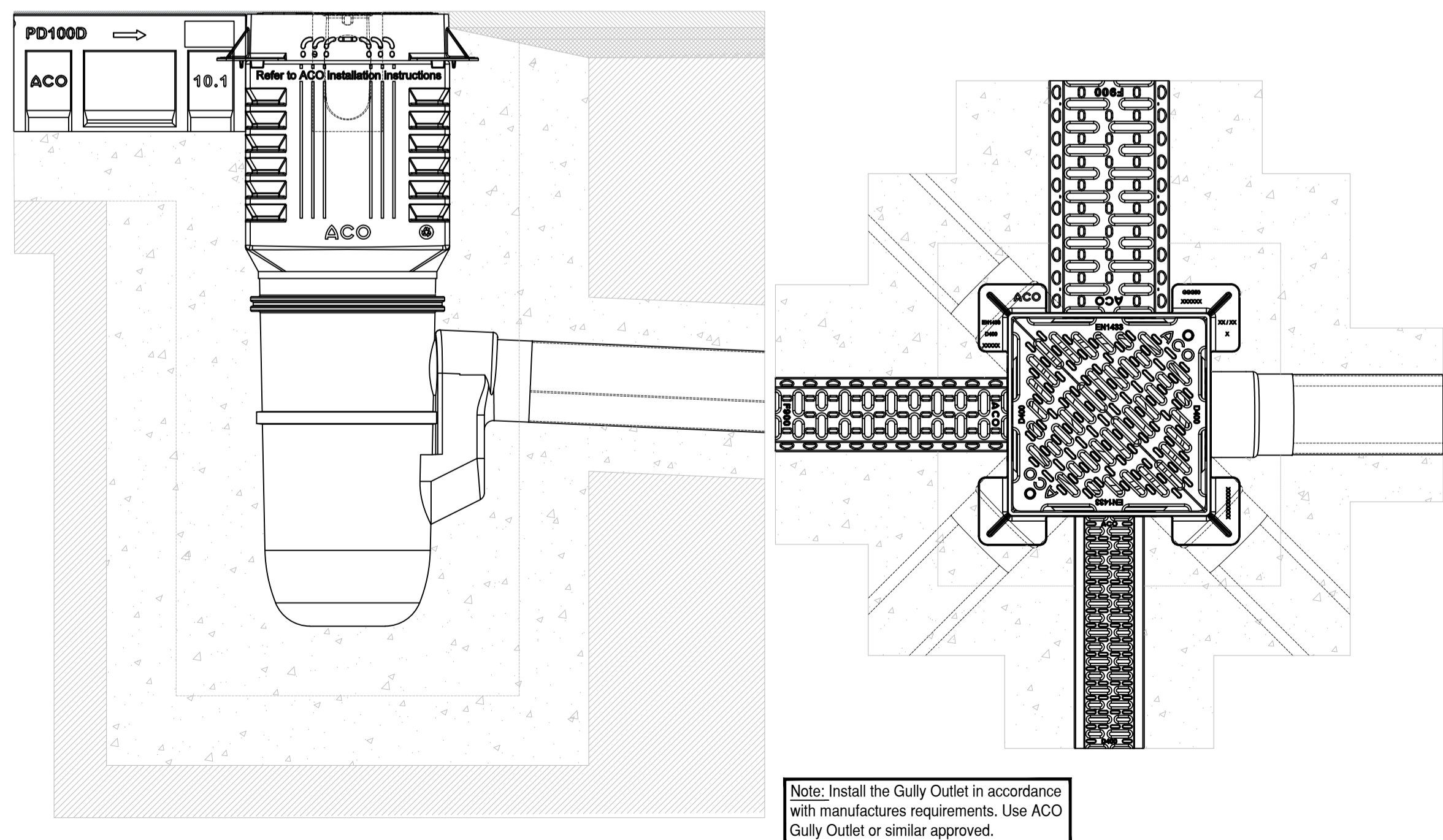
ACO Gully Outlet Details NTS
