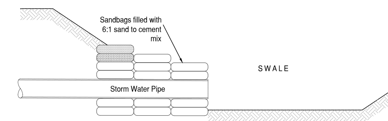
Typical Sandbag Headwall Detail Scale 1:20
