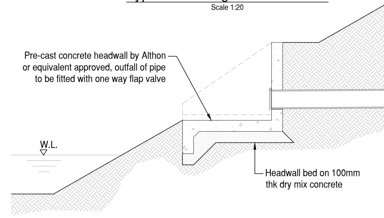
Typical Concrete Headwall Detail Scale 1:20
