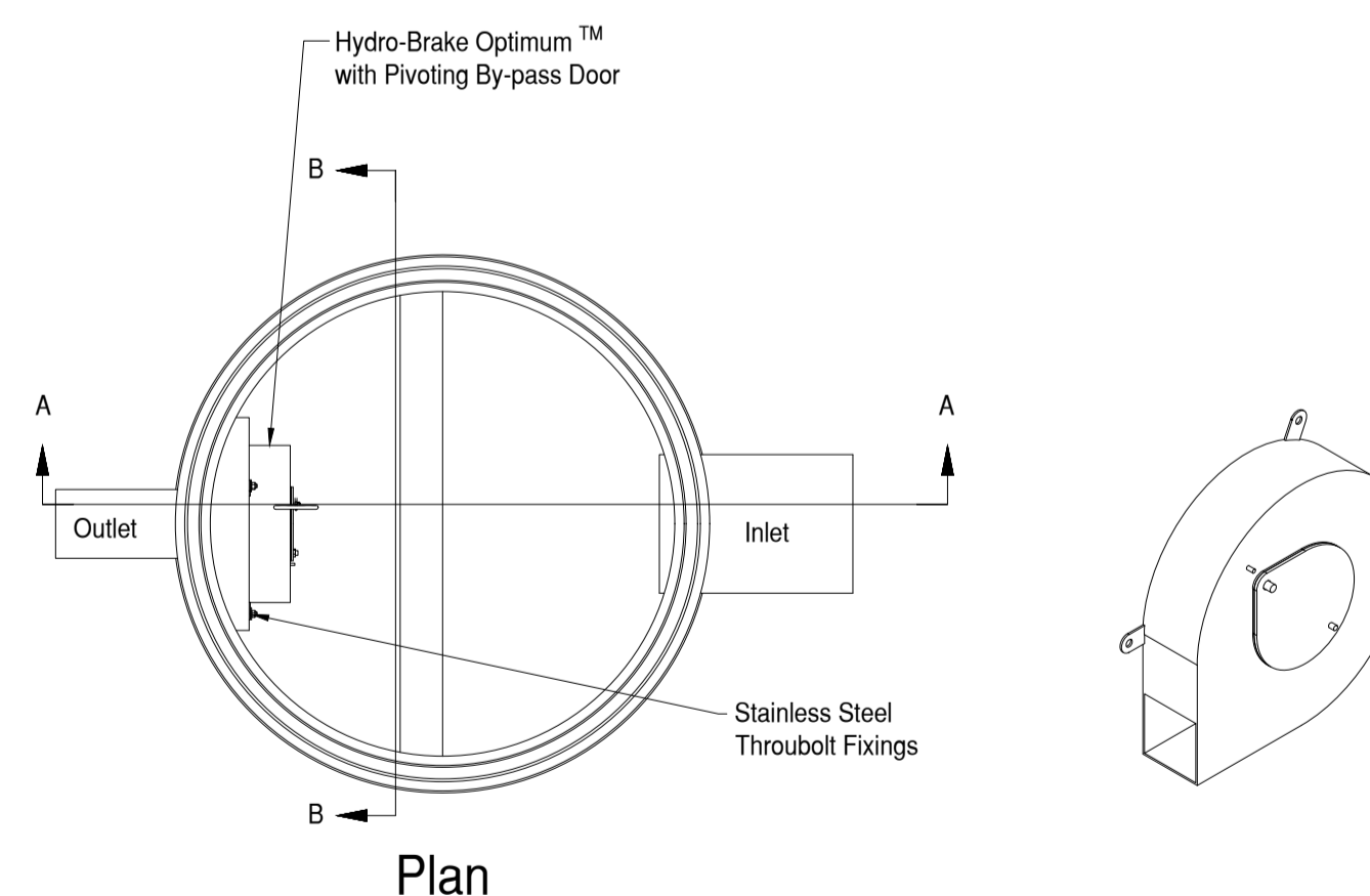
Typical Hydrobrake Chamber Detail With Overflow Pipe Scale 1:20
