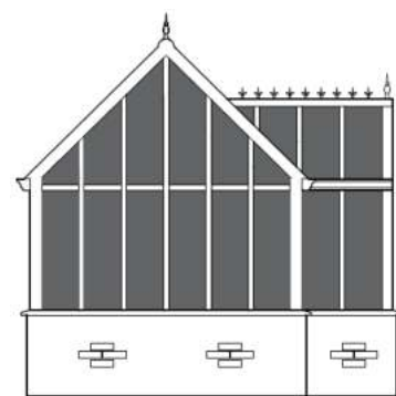
Fig 09: Proposed Side Elevation
