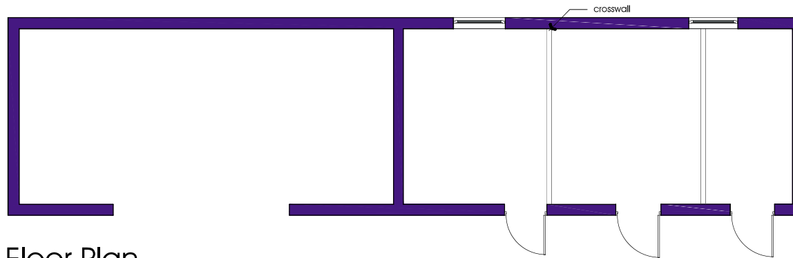
Floor Plan scale 1:100
