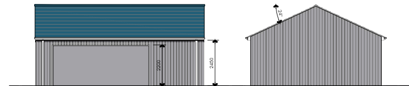
Elevation North East
