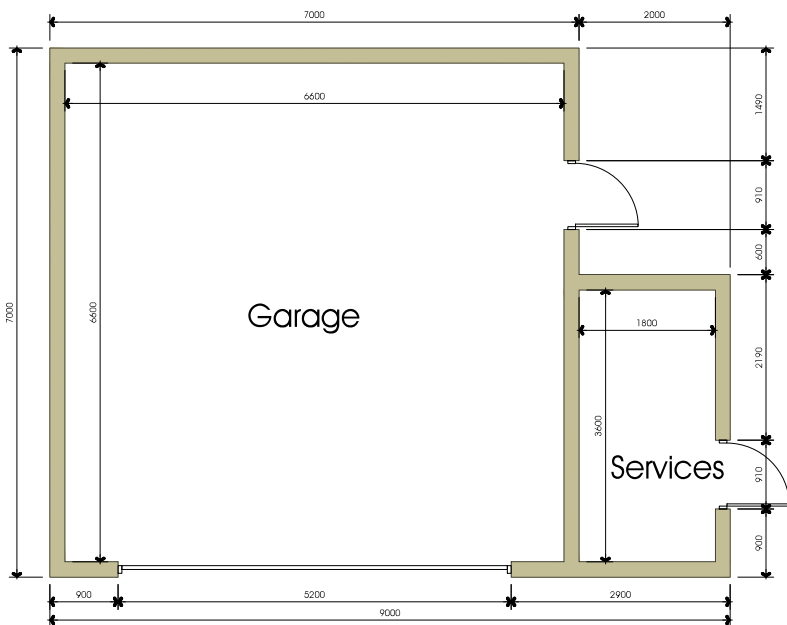
Unit 1 Garage Floor Plan
