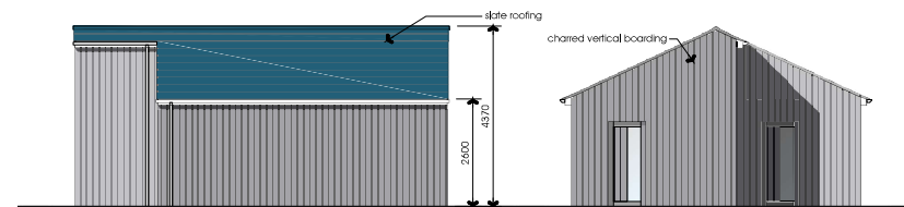
Elevation South West
