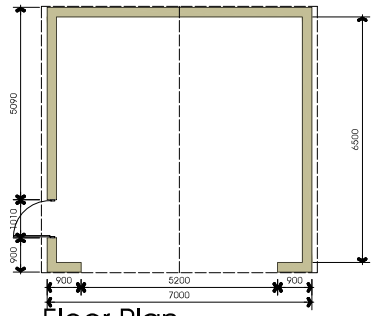
Floor Plan scale 1:100 Garage to Unit 2
