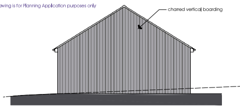
Elevation South East scale 1:100
