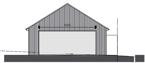
Elevation North West scale 1:100
