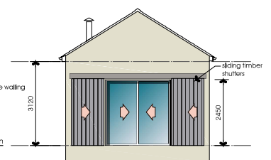
Elevation South West scale 1:100
