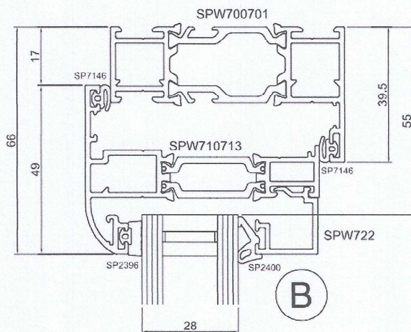
Figure 3 – Vertical section
