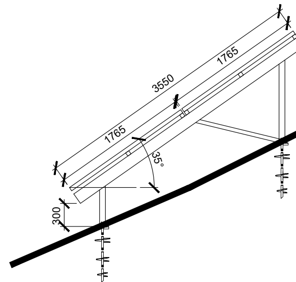
TYPICAL SECTION Solar Panel and ground screw support system
