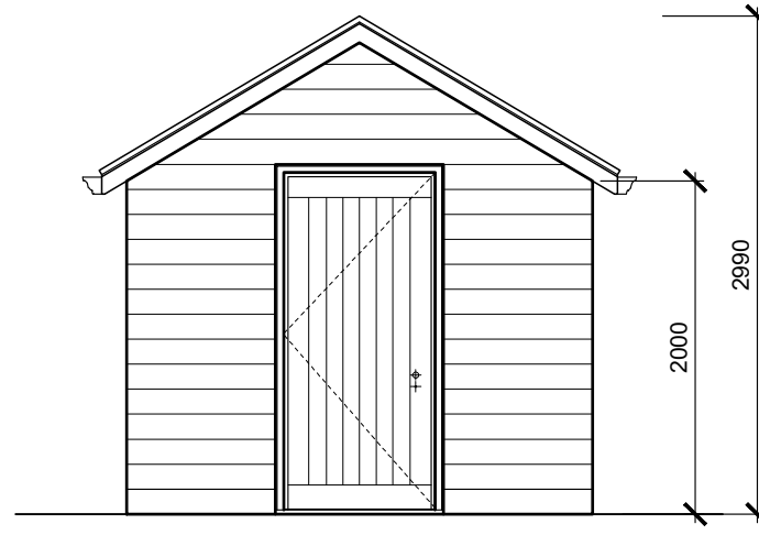
EAST ELEVATION Battery Pack Storage Shed
