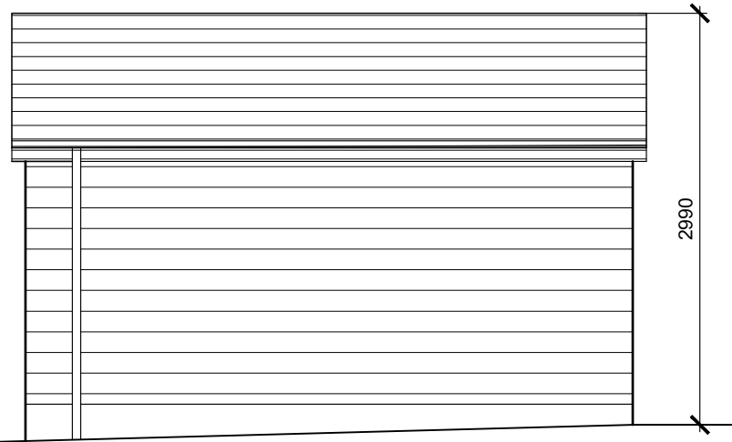
SOUTH ELEVATION Battery Pack Storage Shed
