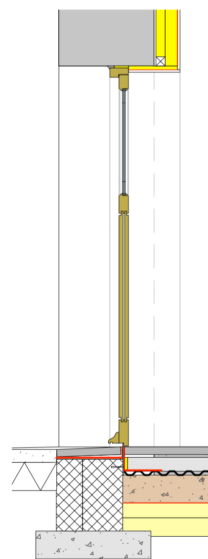
SECTION
