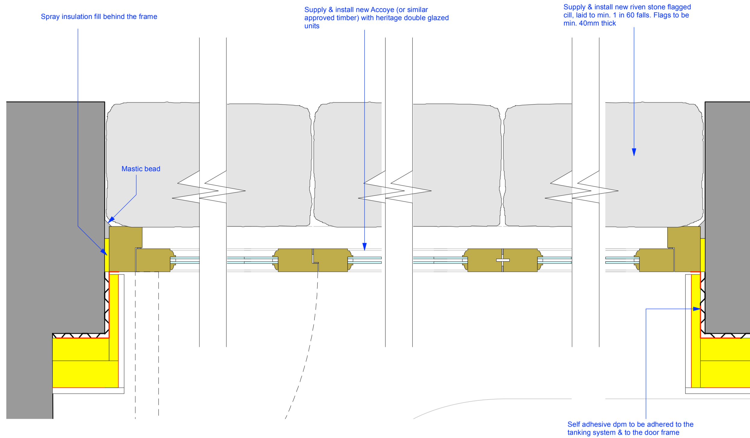
PLAN DETAILS 1:5 SCALE
