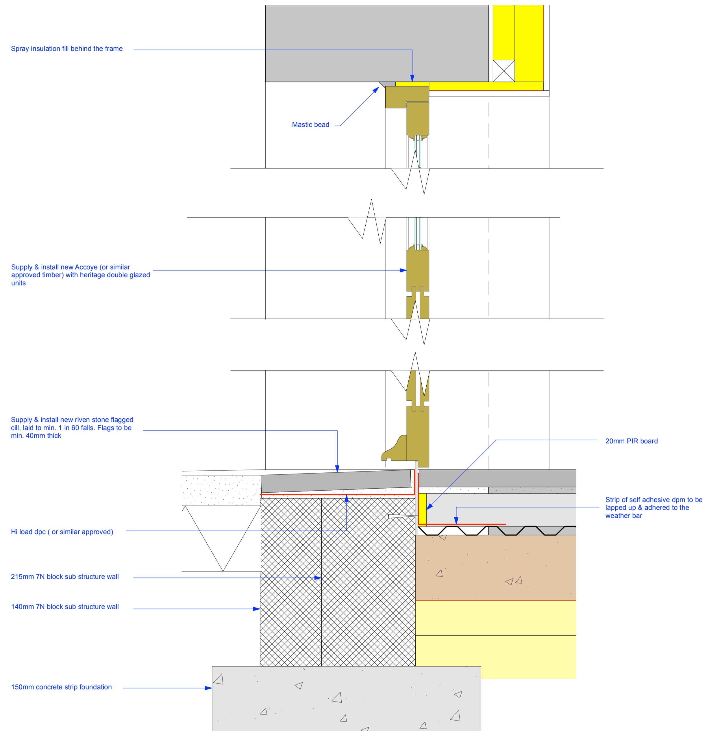
SECTIONAL DETAILS 1:5 SCALE
