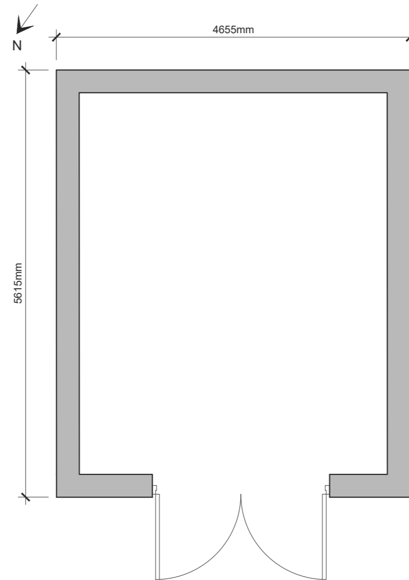
EXISTING FLOOR PLAN Scale 1:50
