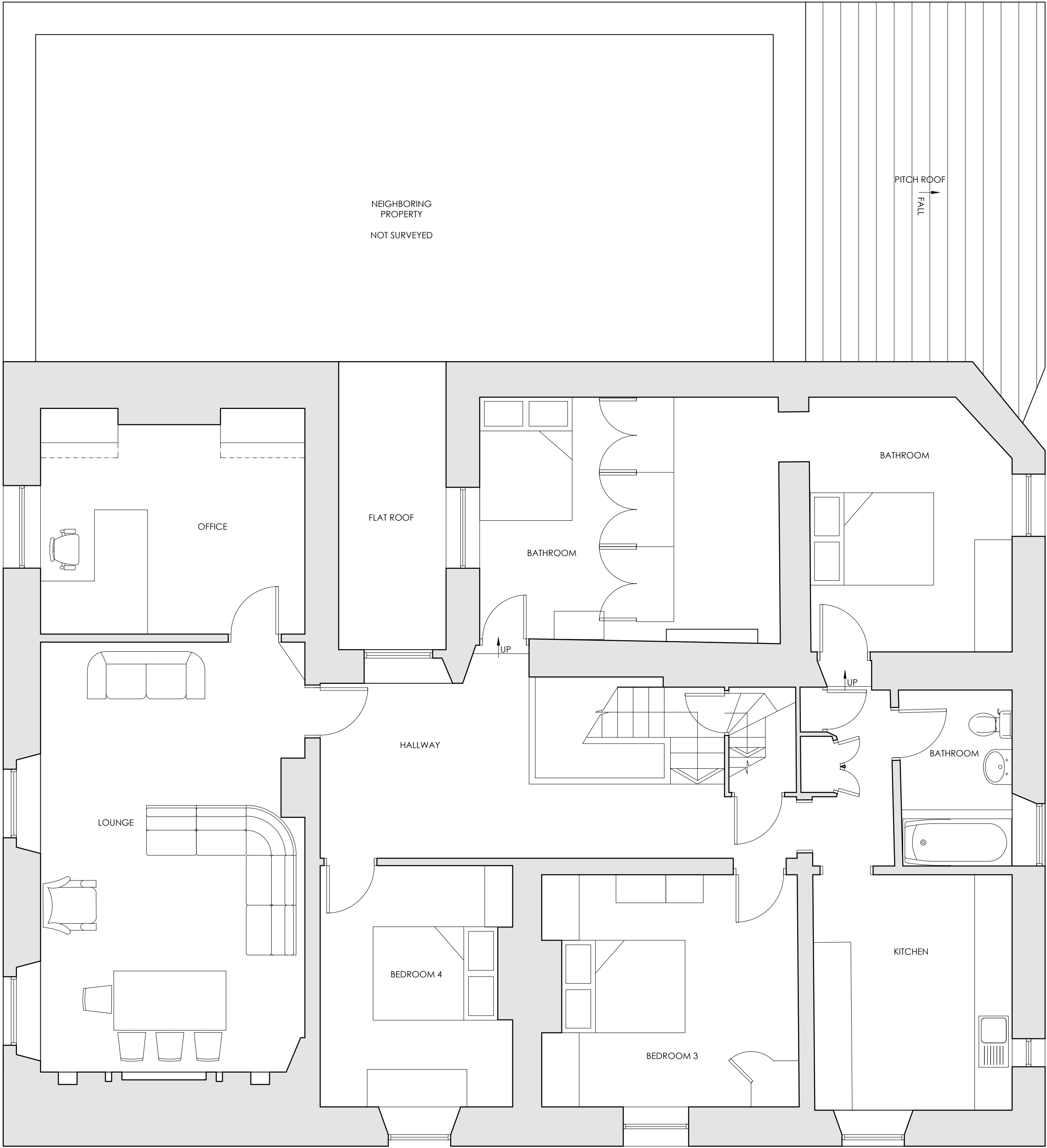
FIRST FLOOR PLAN AS EXISTING 0 1m 2m 3m 4m 5m SCALE
