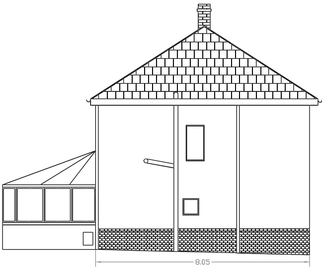
GABLE ELEVATION 1:100
