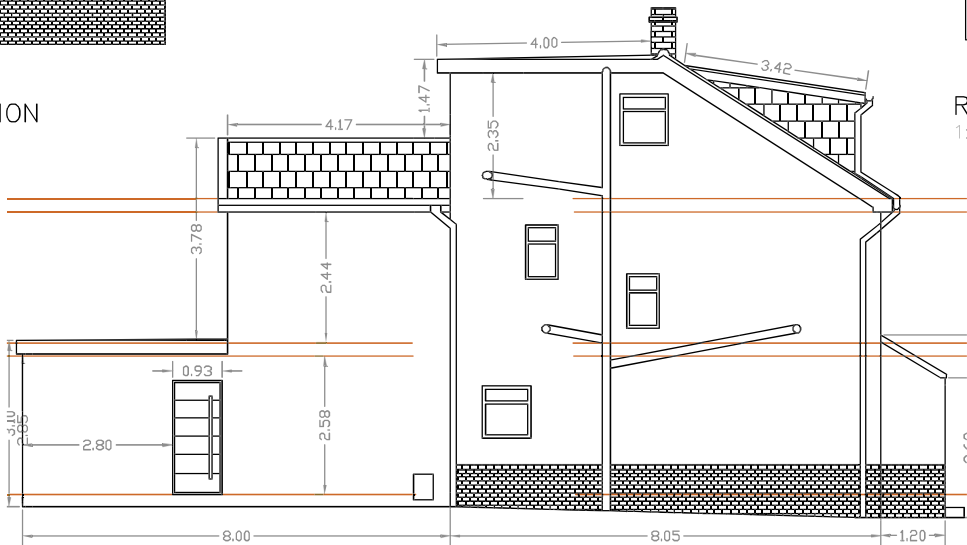
GABLE ELEVATION 1:100
