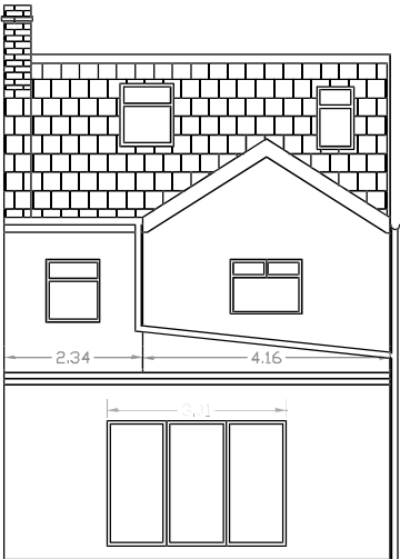
REAR ELEVATION 1:100
