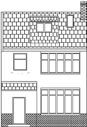
FRONT ELEVATION 1:100
