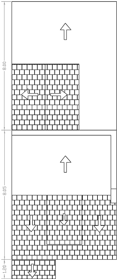
ROOF PLAN 1:100
