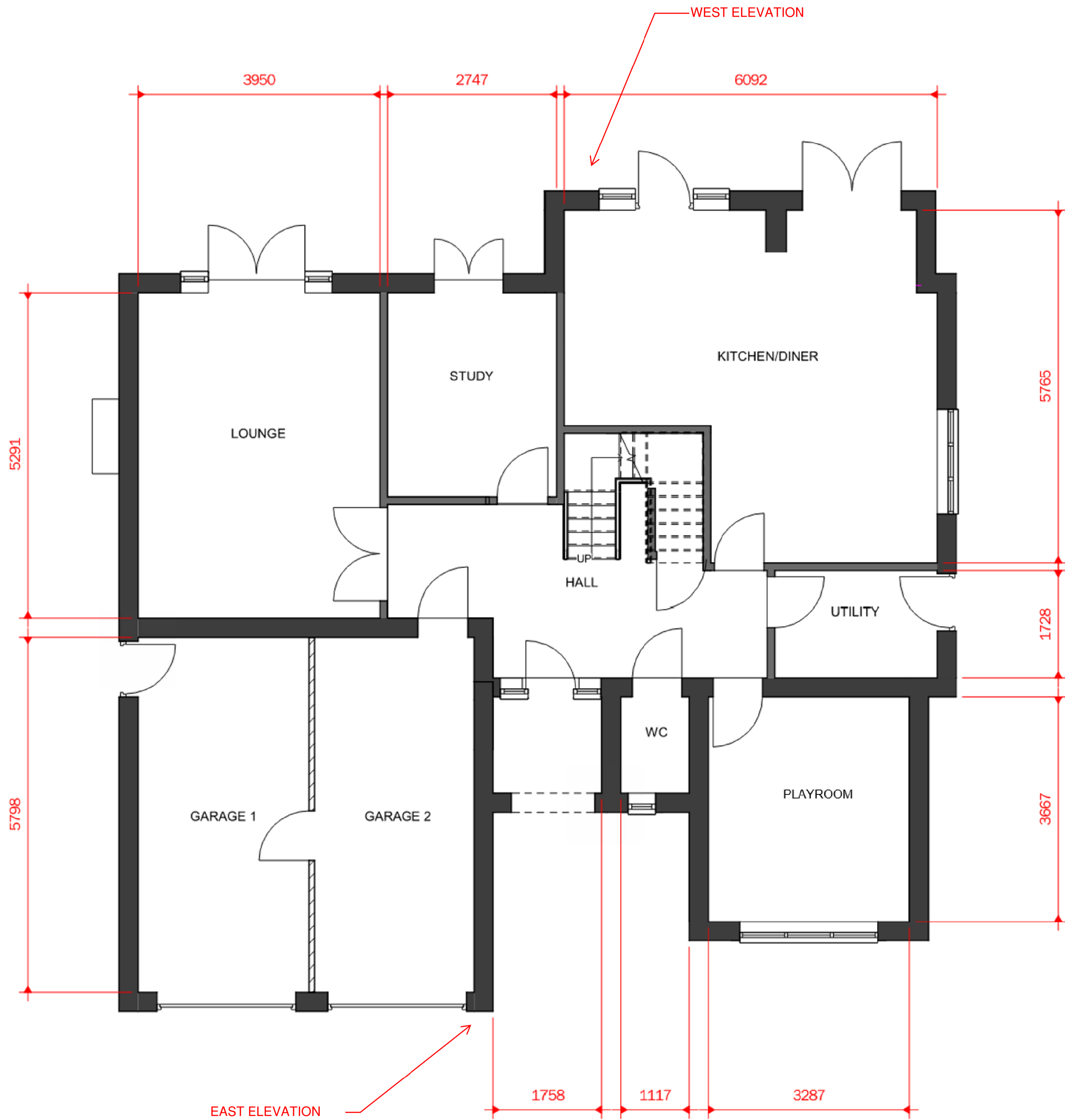
1 0 GROUND FLOOR 1 : 50
