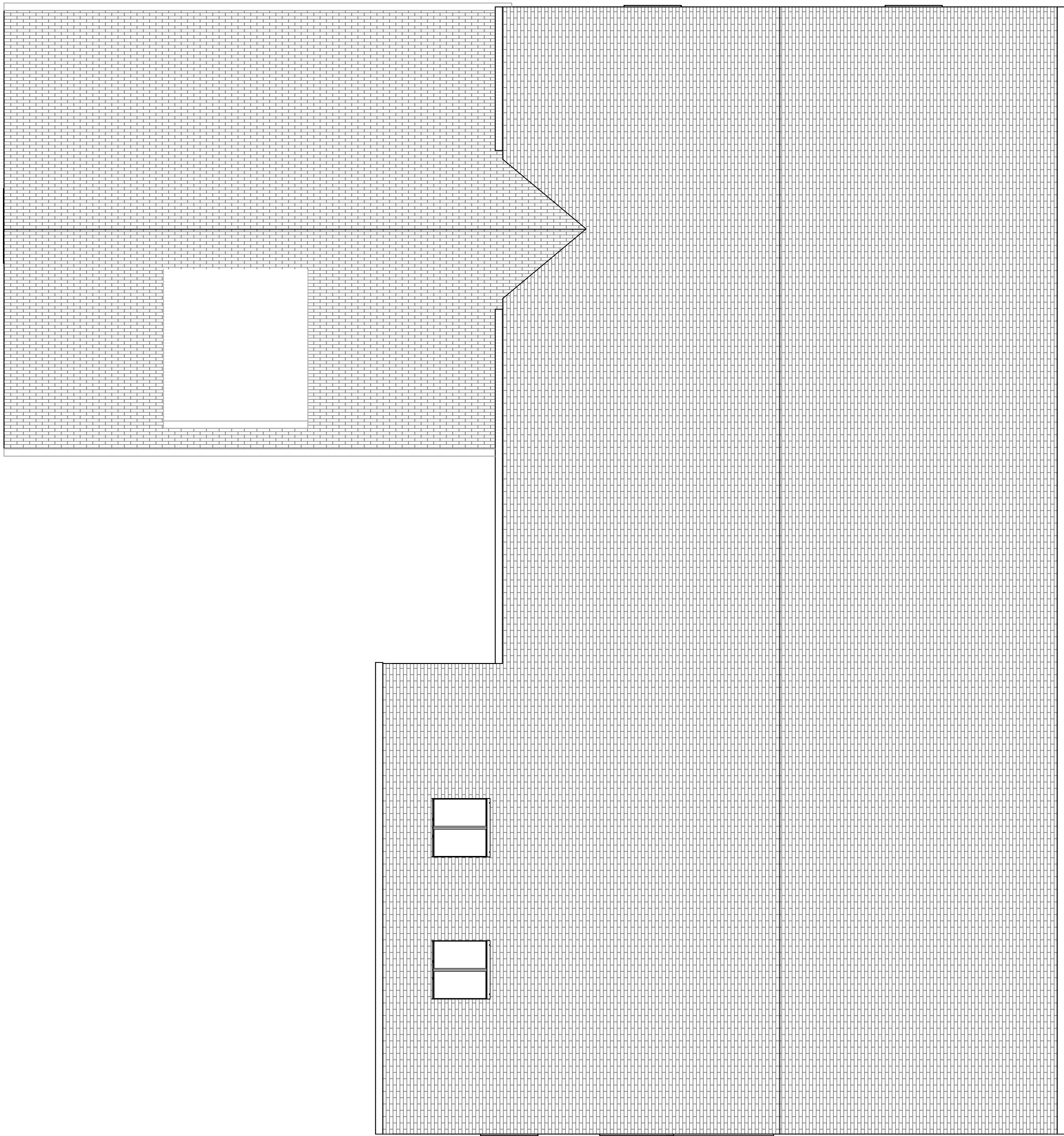
1 Proposed - Roof Plan 1 : 50
