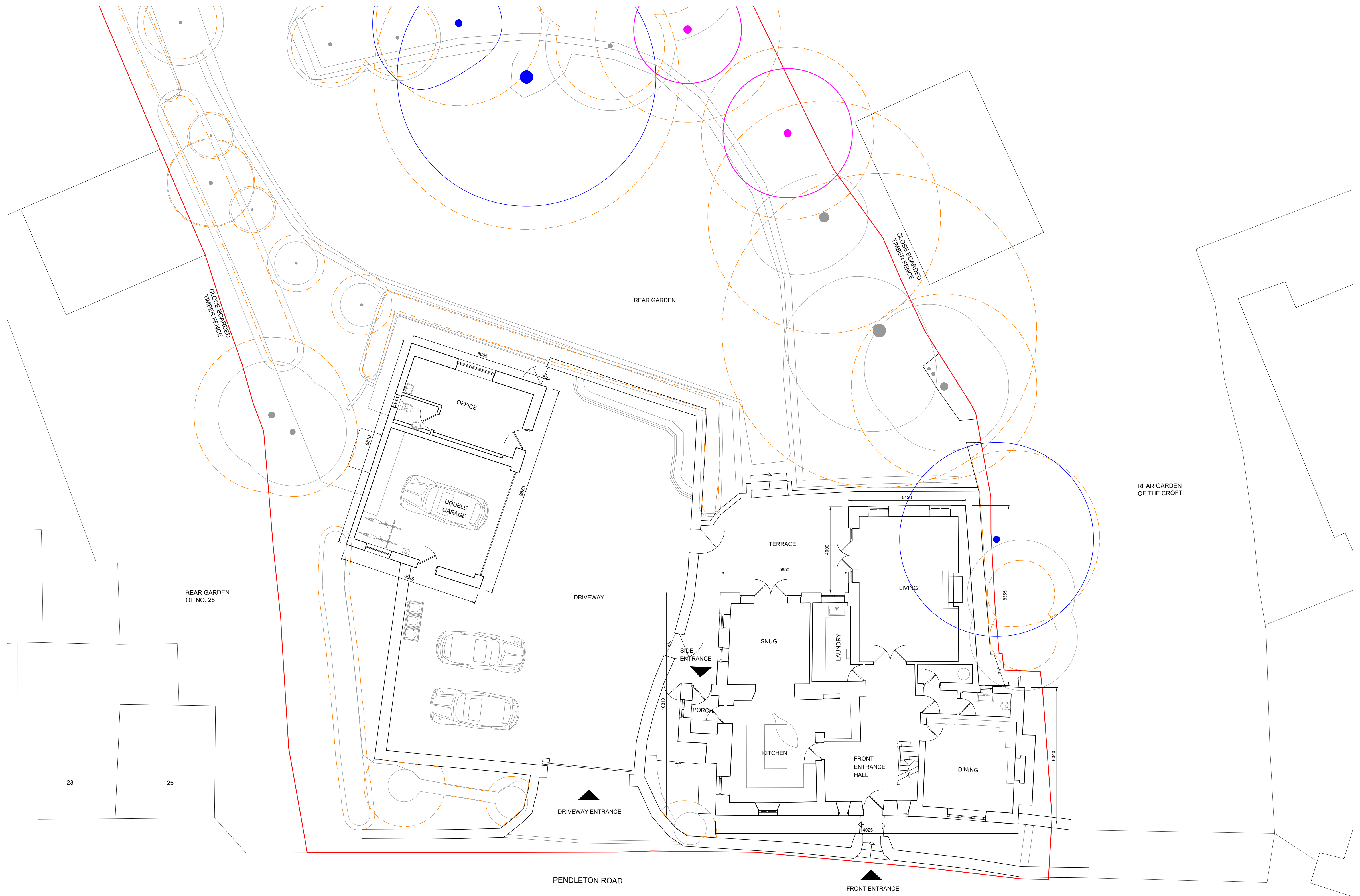
Existing Site Plan - Ground Floor Scale 1:100
