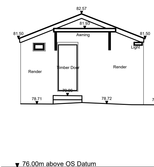
North Elevation
