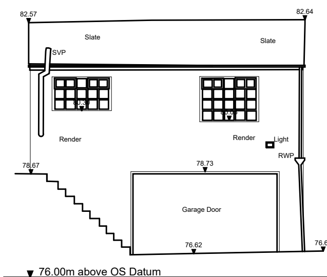
West Elevation
