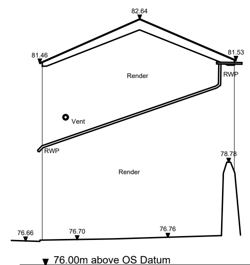
South Elevation
