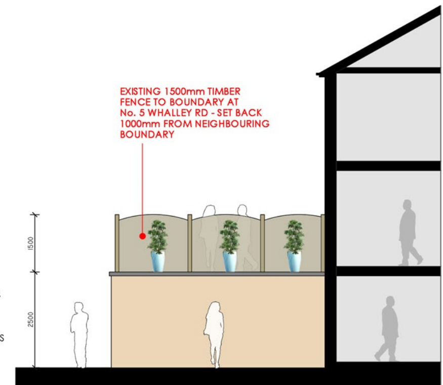
SIDE ELEVATION [No.3] - 1:100 at A3
