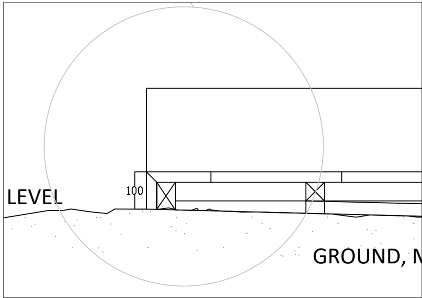
DETAIL 2 (REAR OF PATIO ROAD SIDE) 1:10@A4
