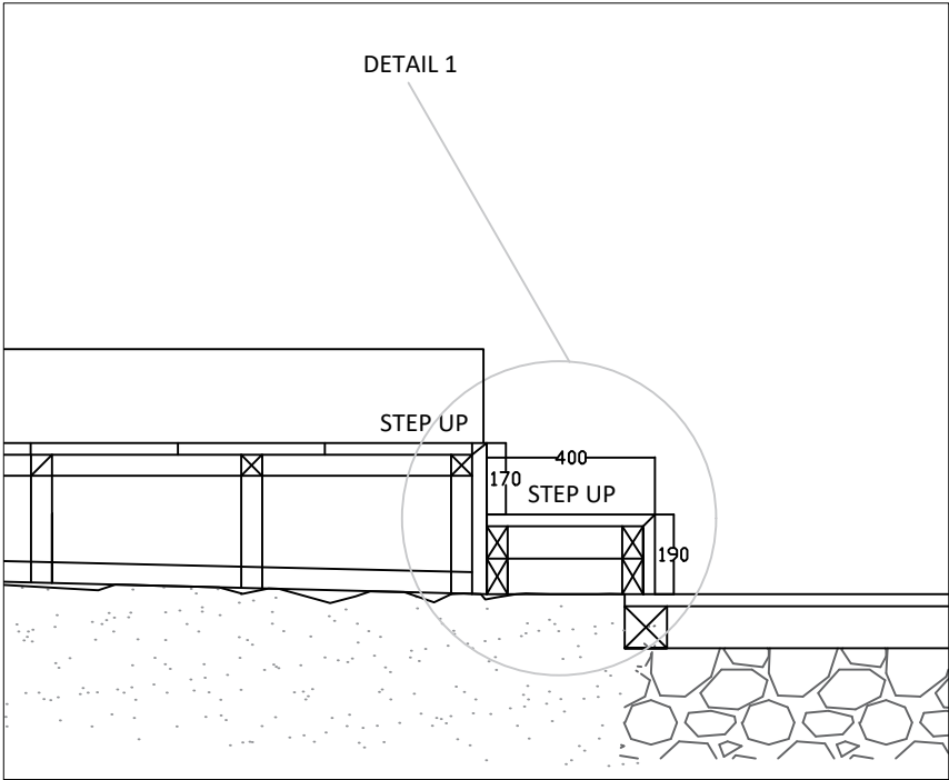
DETAIL 1 (FRONT OF PATIO MARQUEE SIDE) 1:20@A4
