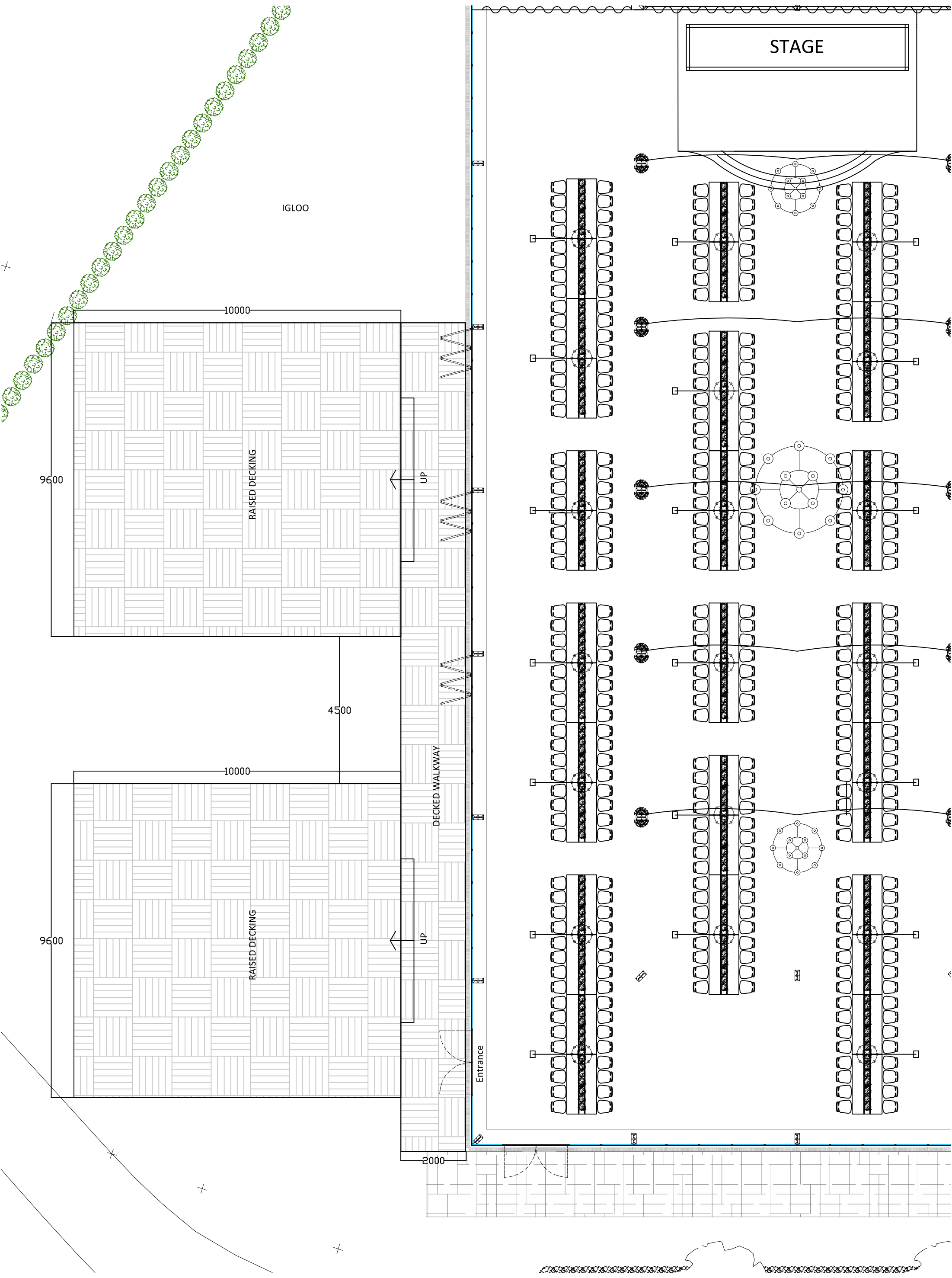
THE GLASS MARQUEE, BLACKBURN A3 @ 1:100 SCALE
