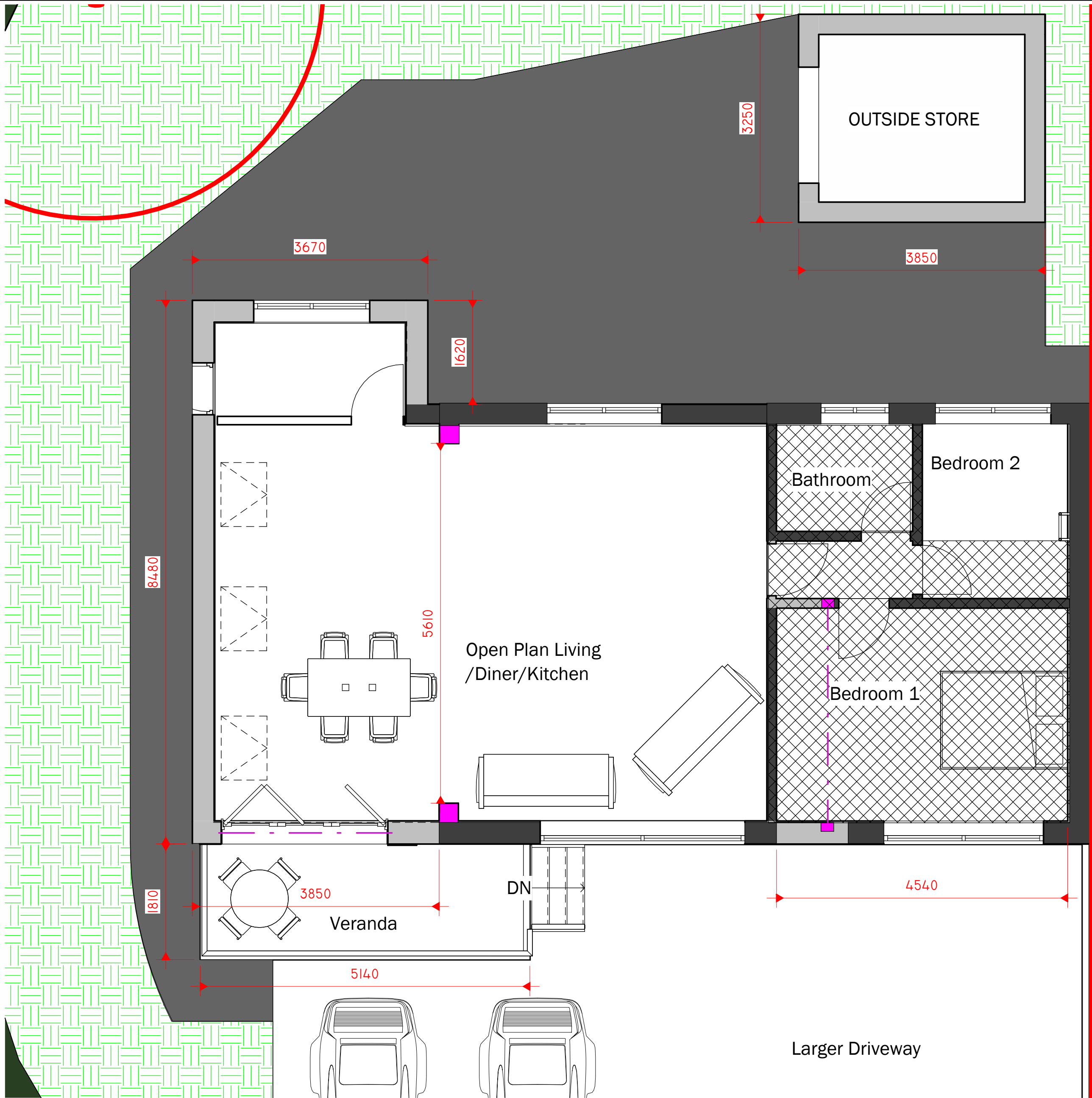
1 0 PROPOSED GROUND FLOOR 1 : 50
