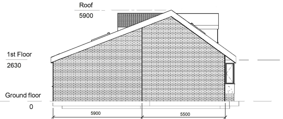
Proposed Side Elevation - LH (4)
