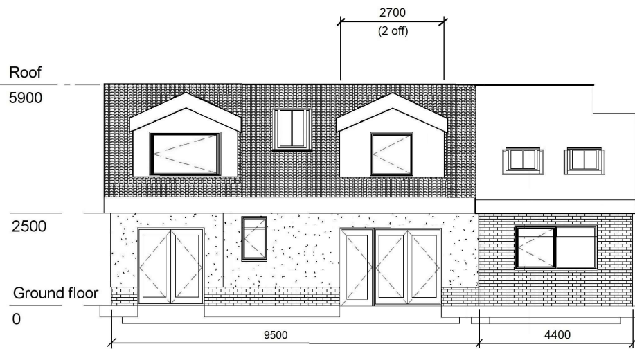
Proposed Rear Elevation (2)
