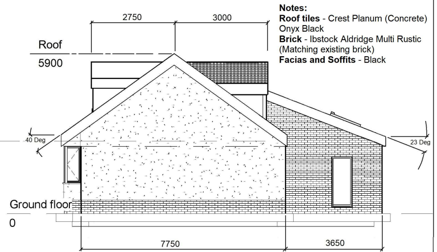
Proposed Side Elevation - RH (3)
