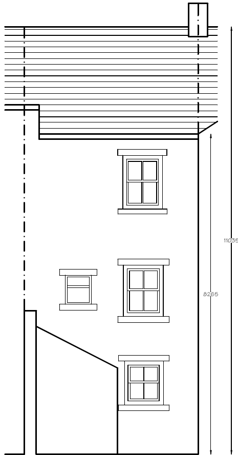
Existing Elevation
