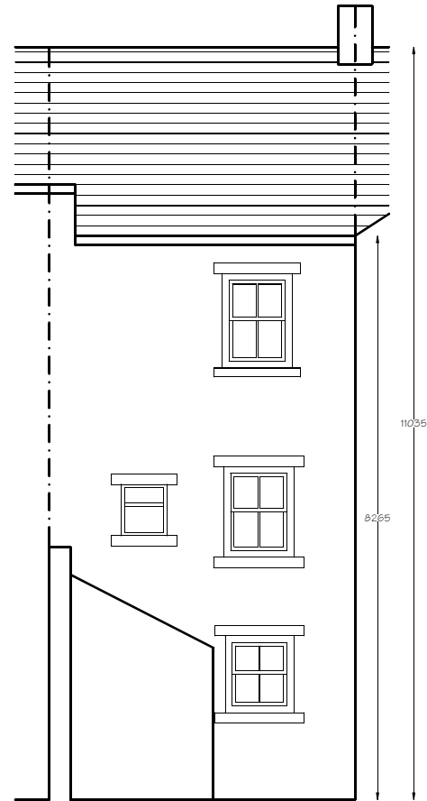
Proposed Elevation
