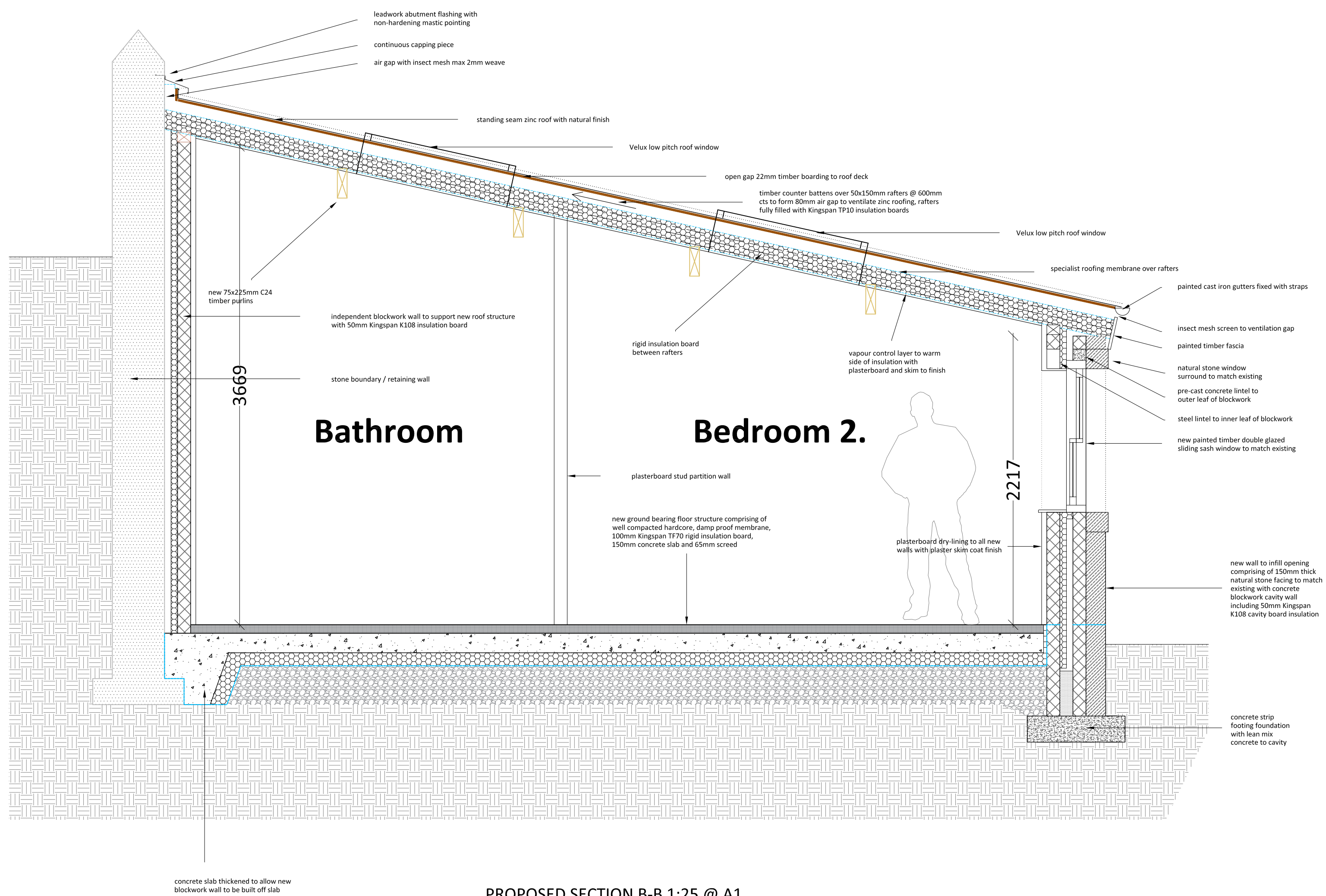
PROPOSED SECTION B-B 1:25 @ A1
