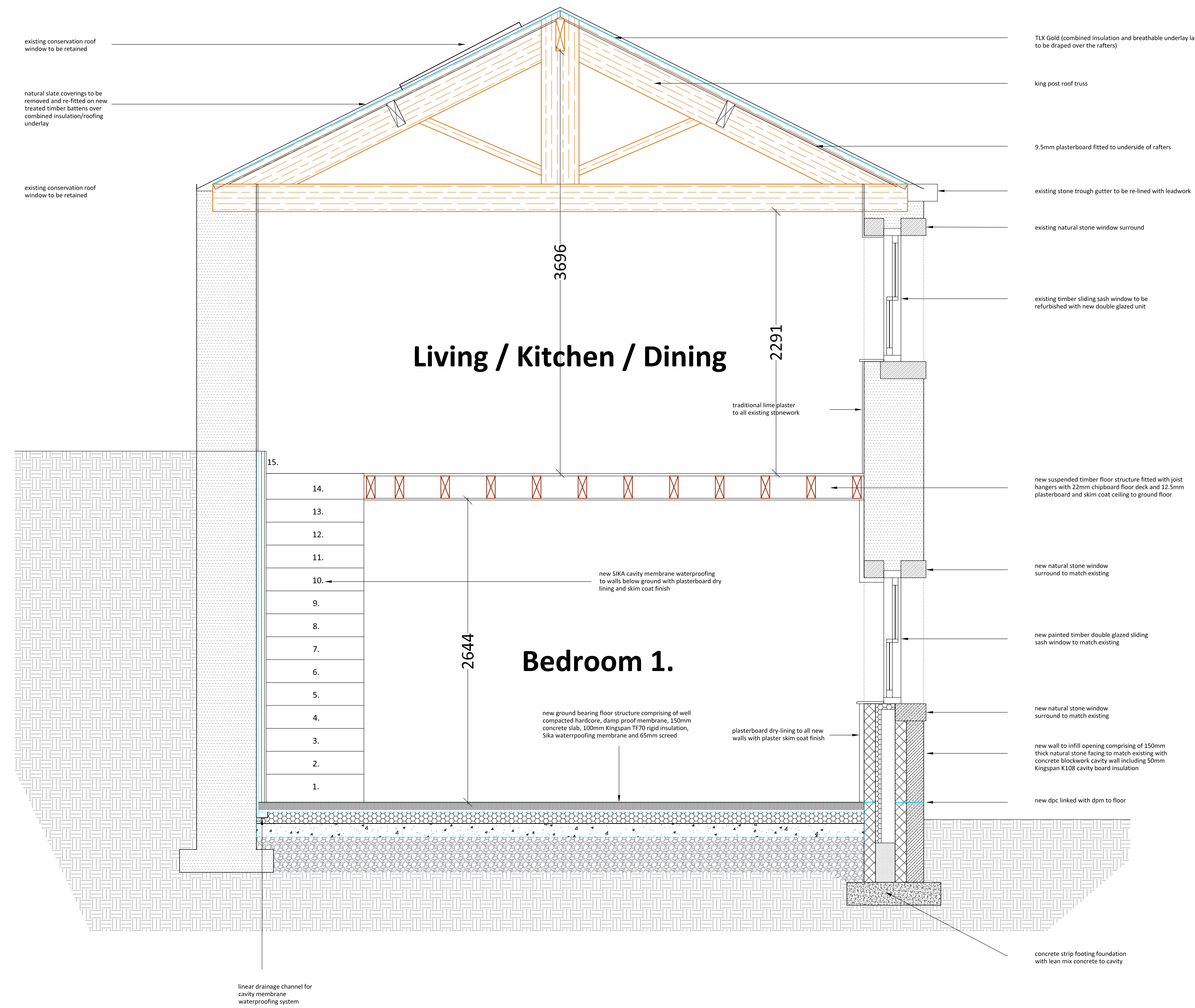
PROPOSED SECTION A-A 1:25 @ A1
