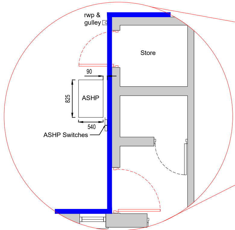
ASHP Plan @ 1:50
