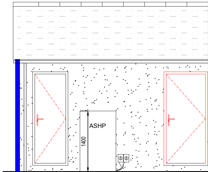
ASHP Elevation @ 1:50
