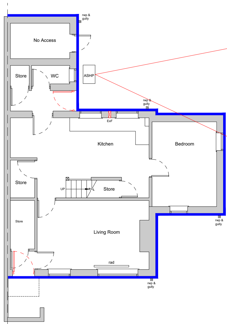
Proposed GA Floor Plan @ 1:100
