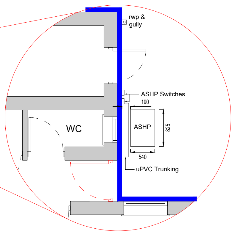
ASHP Plan @ 1:50
