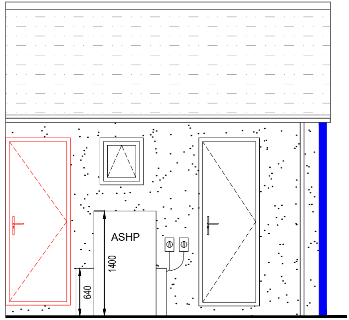
ASHP Elevation @ 1:50
